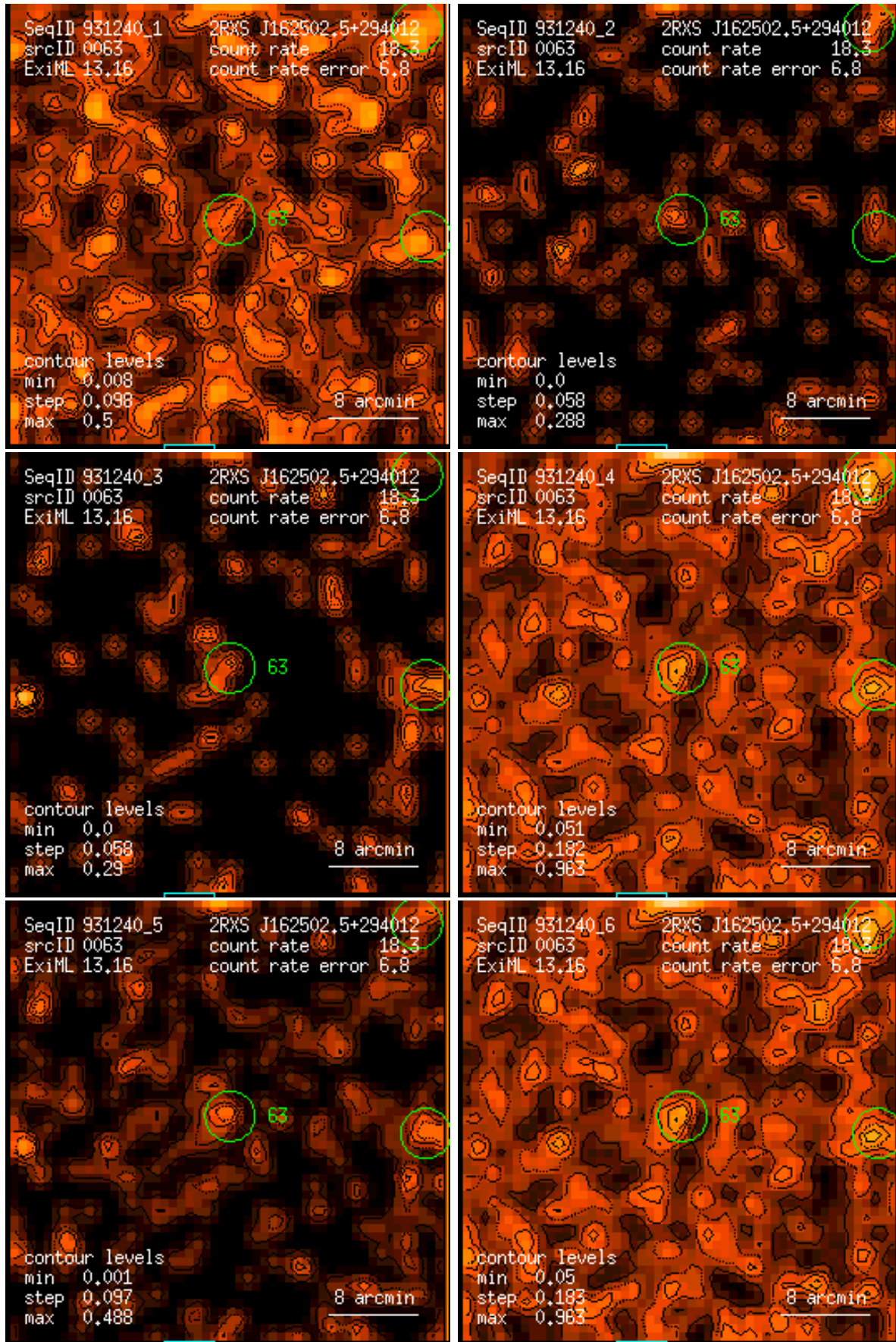
Figure 63: RASS 931240: detection 0063: band rate images, Gaussian filter: (1) PSPC channels 11 – 41, (2) 52 – 90, (3) 91 – 201, (4) 11 – 235, (5) 52 – 201, (6) 11 – 201. Broad band rates in counts/ks. Band rate contour levels in counts/ks/arcmin 2 .
