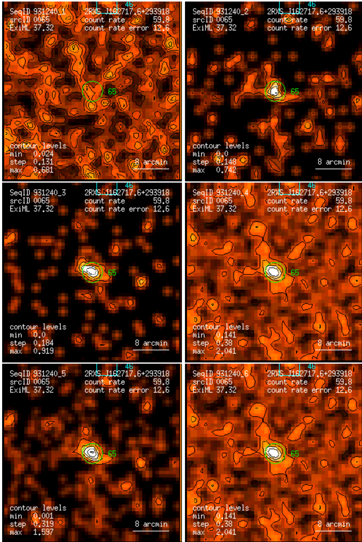
Figure 65: RASS 931240: detection 0065: band rate images, Gaussian filter: (1) PSPC channels 11 – 41, (2) 52 – 90, (3) 91 – 201, (4) 11 – 235, (5) 52 – 201, (6) 11 – 201. Broad band rates in counts/ks. Band rate contour levels in counts/ks/arcmin 2 .
