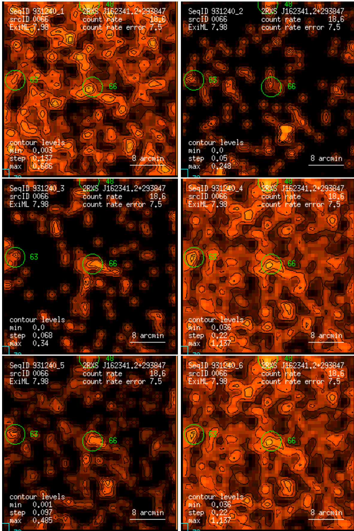
Figure 66: RASS 931240: detection 0066: band rate images, Gaussian filter: (1) PSPC channels 11 – 41, (2) 52 – 90, (3) 91 – 201, (4) 11 – 235, (5) 52 – 201, (6) 11 – 201. Broad band rates in counts/ks. Band rate contour levels in counts/ks/arcmin 2 .
