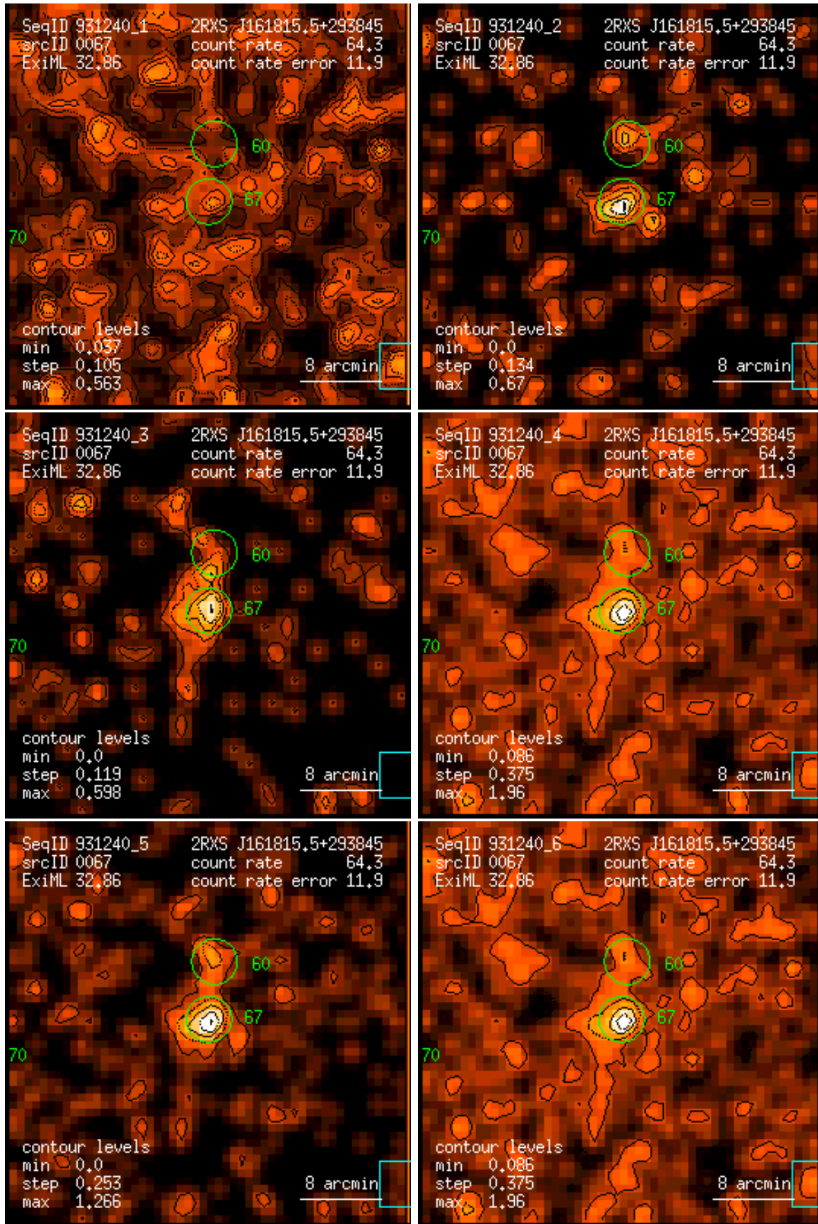
Figure 67: RASS 931240: detection 0067: band rate images, Gaussian filter: (1) PSPC channels 11 – 41, (2) 52 – 90, (3) 91 – 201, (4) 11 – 235, (5) 52 – 201, (6) 11 – 201. Broad band rates in counts/ks. Band rate contour levels in counts/ks/arcmin 2 .
