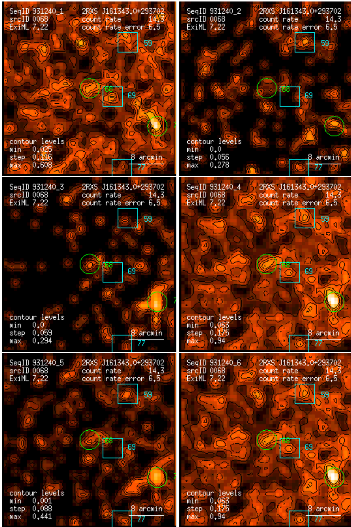
Figure 68: RASS 931240: detection 0068: band rate images, Gaussian filter: (1) PSPC channels 11 – 41, (2) 52 – 90, (3) 91 – 201, (4) 11 – 235, (5) 52 – 201, (6) 11 – 201. Broad band rates in counts/ks. Band rate contour levels in counts/ks/arcmin 2 .
