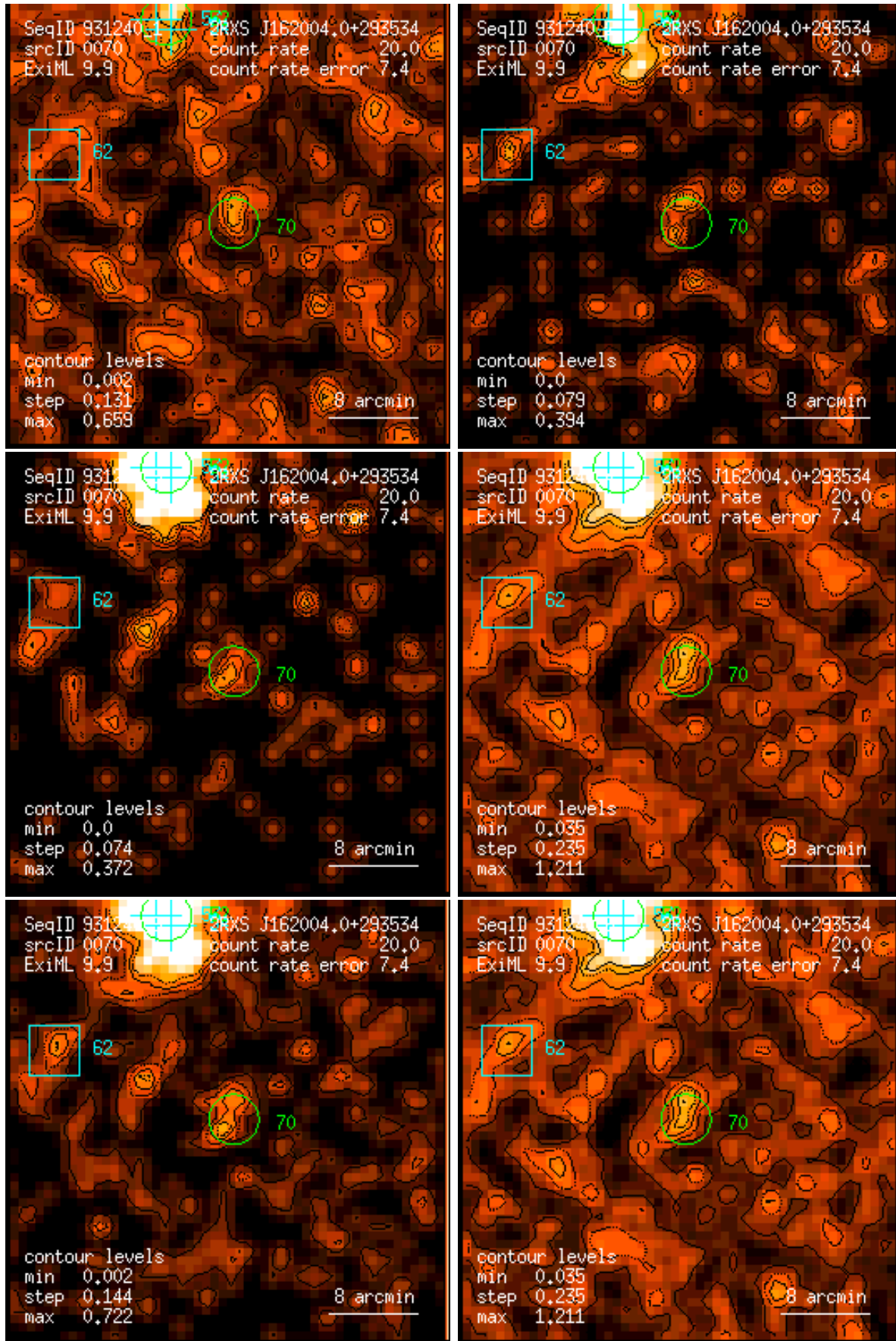
Figure 70: RASS 931240: detection 0070: band rate images, Gaussian filter: (1) PSPC channels 11 – 41, (2) 52 – 90, (3) 91 – 201, (4) 11 – 235, (5) 52 – 201, (6) 11 – 201. Broad band rates in counts/ks. Band rate contour levels in counts/ks/arcmin 2 .
