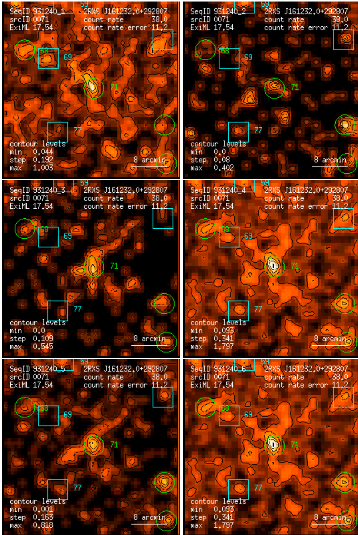
Figure 71: RASS 931240: detection 0071: band rate images, Gaussian filter: (1) PSPC channels 11 – 41, (2) 52 – 90, (3) 91 – 201, (4) 11 – 235, (5) 52 – 201, (6) 11 – 201. Broad band rates in counts/ks. Band rate contour levels in counts/ks/arcmin 2 .
