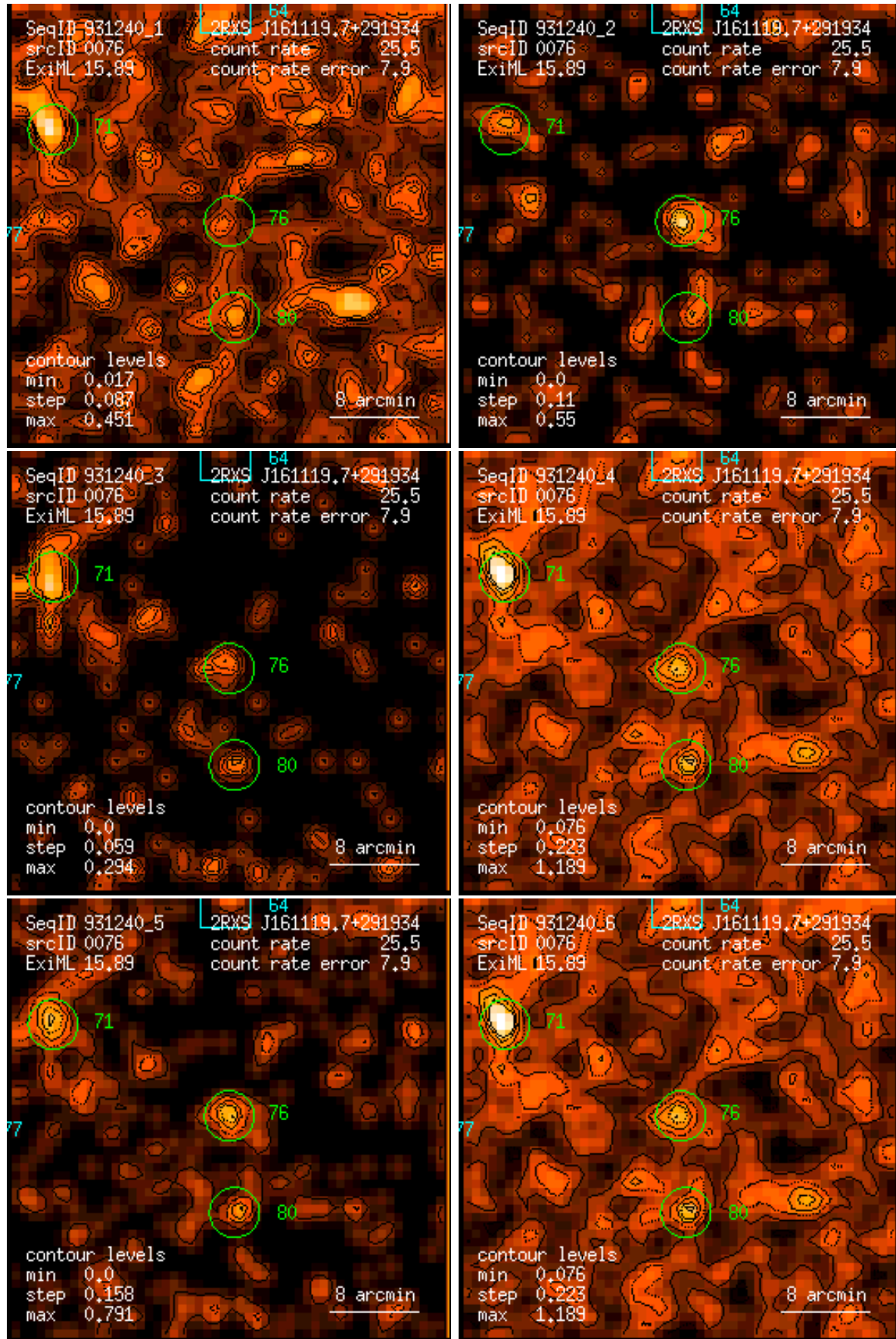
Figure 76: RASS 931240: detection 0076: band rate images, Gaussian filter: (1) PSPC channels 11 – 41, (2) 52 – 90, (3) 91 – 201, (4) 11 – 235, (5) 52 – 201, (6) 11 – 201. Broad band rates in counts/ks. Band rate contour levels in counts/ks/arcmin 2 .
