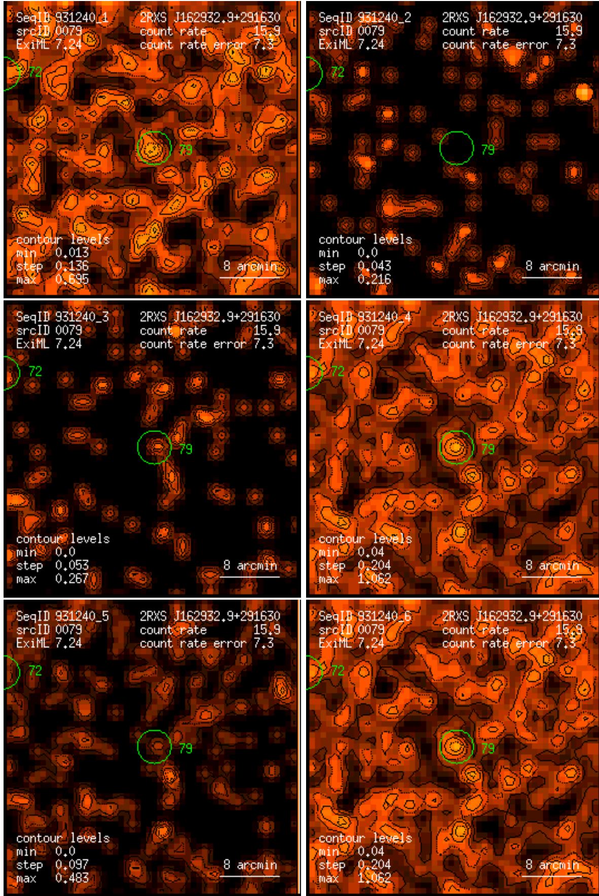
Figure 79: RASS 931240: detection 0079: band rate images, Gaussian filter: (1) PSPC channels 11 – 41, (2) 52 – 90, (3) 91 – 201, (4) 11 – 235, (5) 52 – 201, (6) 11 – 201. Broad band rates in counts/ks. Band rate contour levels in counts/ks/arcmin 2 .
