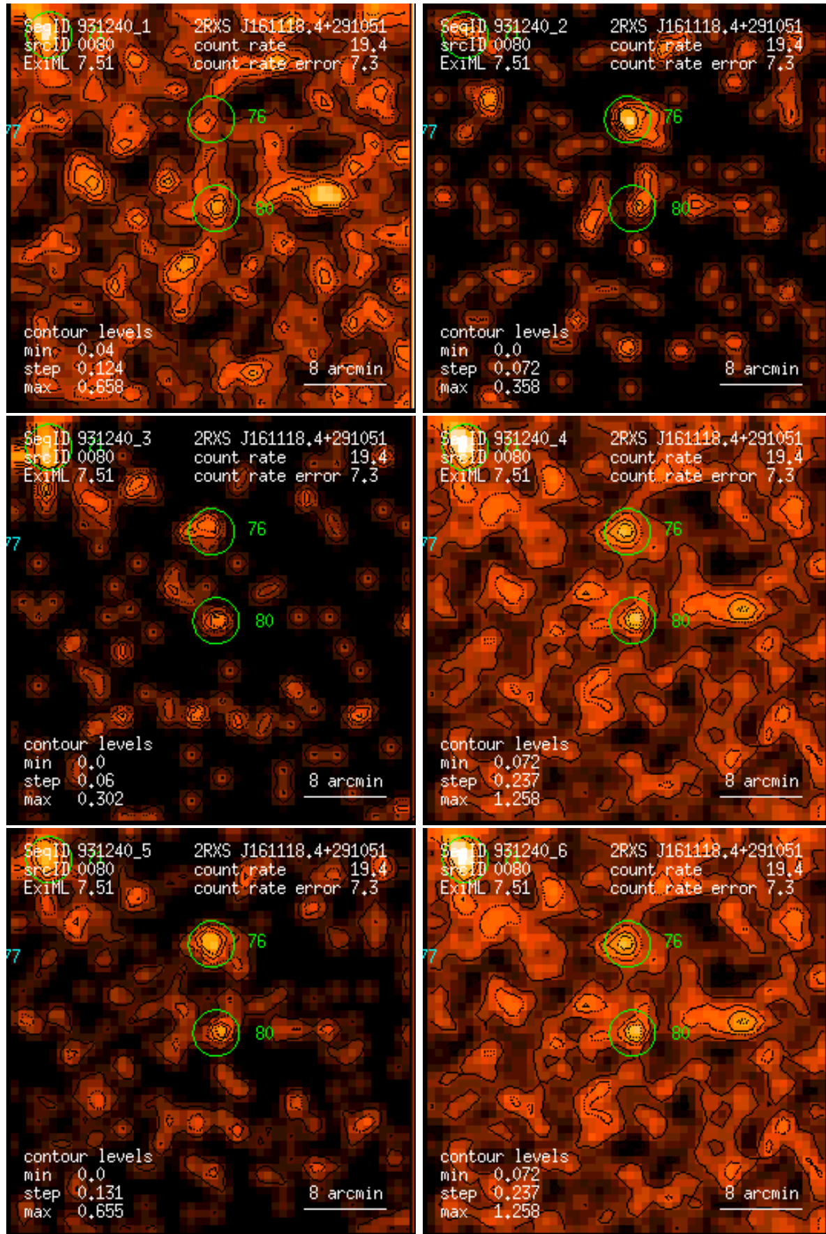
Figure 80: RASS 931240: detection 0080: band rate images, Gaussian filter: (1) PSPC channels 11 – 41, (2) 52 – 90, (3) 91 – 201, (4) 11 – 235, (5) 52 – 201, (6) 11 – 201. Broad band rates in counts/ks. Band rate contour levels in counts/ks/arcmin 2 .
