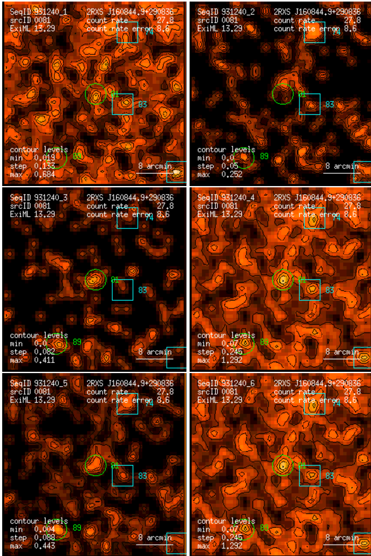
Figure 81: RASS 931240: detection 0081: band rate images, Gaussian filter: (1) PSPC channels 11 – 41, (2) 52 – 90, (3) 91 – 201, (4) 11 – 235, (5) 52 – 201, (6) 11 – 201. Broad band rates in counts/ks. Band rate contour levels in counts/ks/arcmin 2 .
