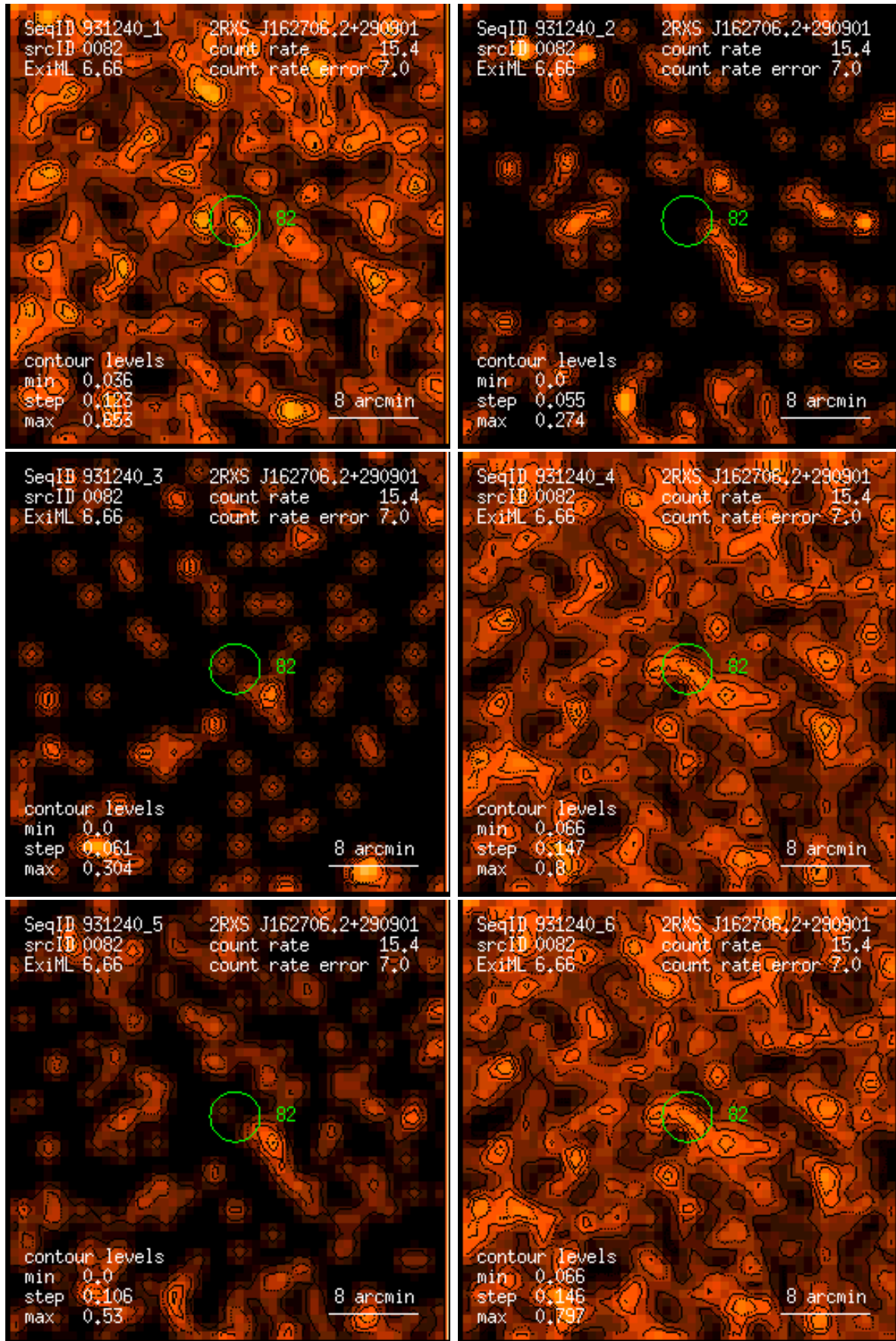
Figure 82: RASS 931240: detection 0082: band rate images, Gaussian filter: (1) PSPC channels 11 – 41, (2) 52 – 90, (3) 91 – 201, (4) 11 – 235, (5) 52 – 201, (6) 11 – 201. Broad band rates in counts/ks. Band rate contour levels in counts/ks/arcmin 2 .
