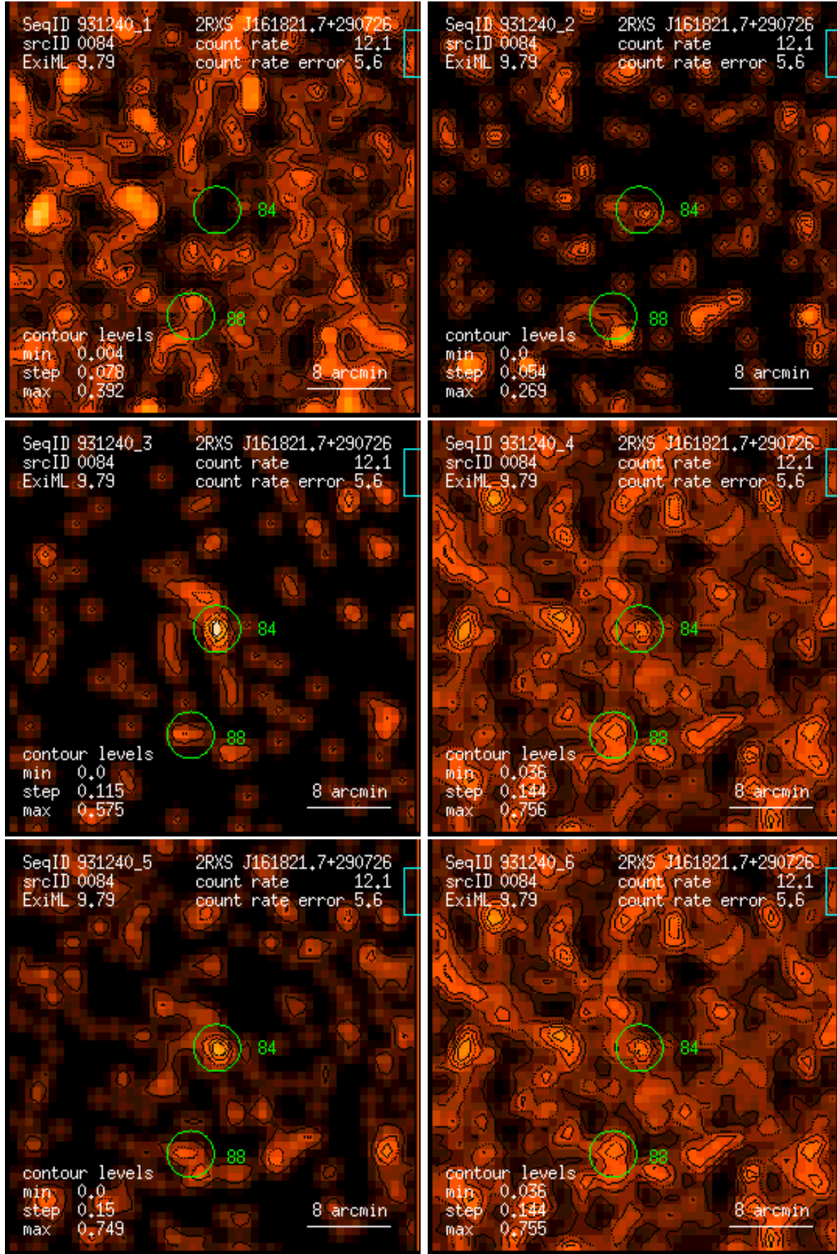
Figure 84: RASS 931240: detection 0084: band rate images, Gaussian filter: (1) PSPC channels 11 – 41, (2) 52 – 90, (3) 91 – 201, (4) 11 – 235, (5) 52 – 201, (6) 11 – 201. Broad band rates in counts/ks. Band rate contour levels in counts/ks/arcmin 2 .
