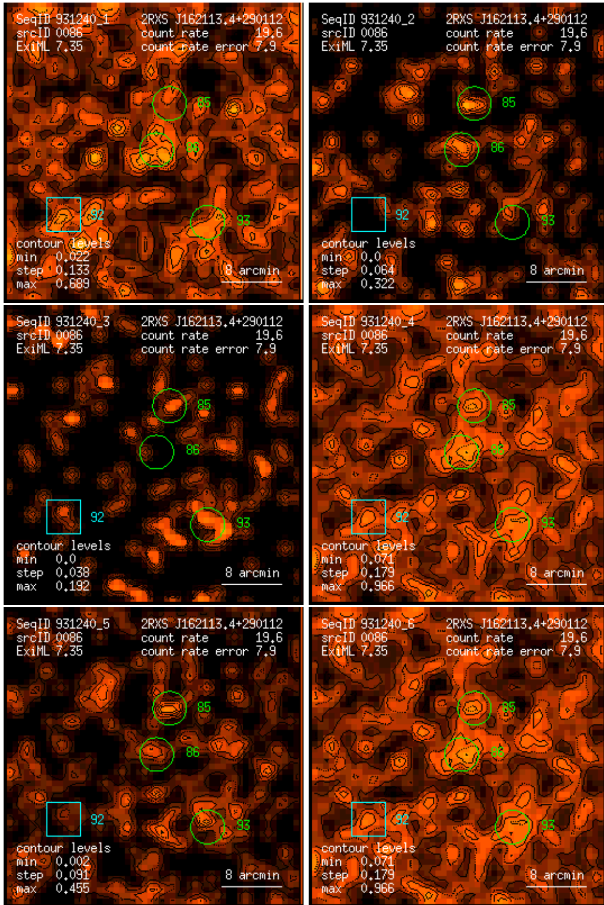
Figure 86: RASS 931240: detection 0086: band rate images, Gaussian filter: (1) PSPC channels 11 – 41, (2) 52 – 90, (3) 91 – 201, (4) 11 – 235, (5) 52 – 201, (6) 11 – 201. Broad band rates in counts/ks. Band rate contour levels in counts/ks/arcmin 2 .
