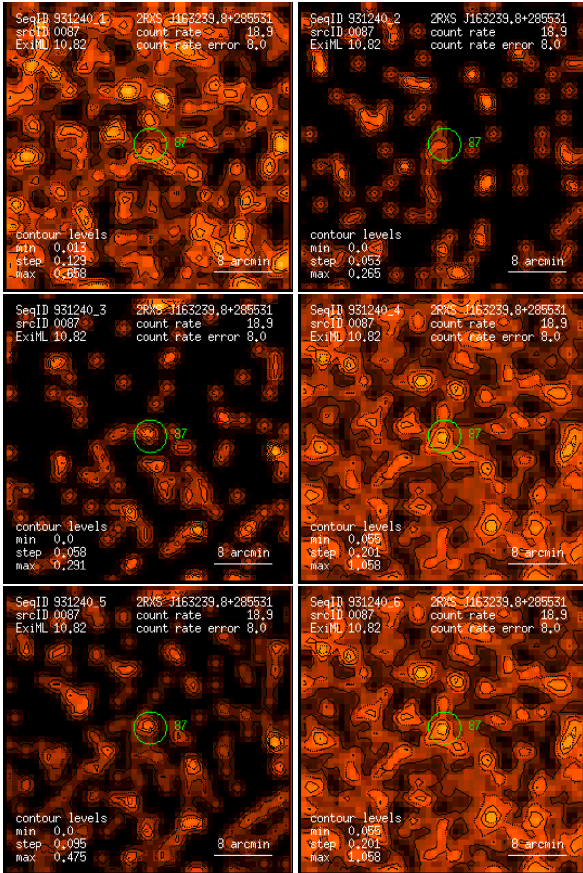
Figure 87: RASS 931240: detection 0087: band rate images, Gaussian filter: (1) PSPC channels 11 – 41, (2) 52 – 90, (3) 91 – 201, (4) 11 – 235, (5) 52 – 201, (6) 11 – 201. Broad band rates in counts/ks. Band rate contour levels in counts/ks/arcmin 2 .
