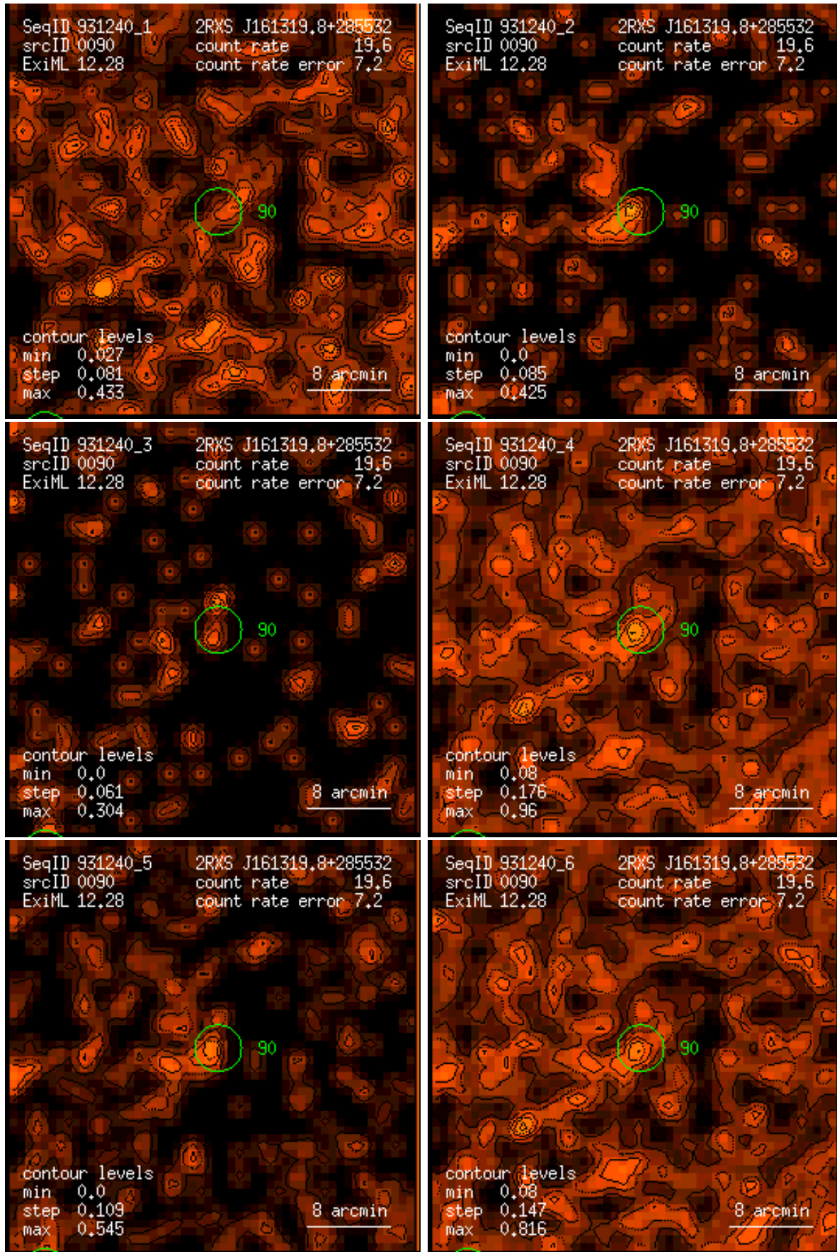
Figure 90: RASS 931240: detection 0090: band rate images, Gaussian filter: (1) PSPC channels 11 – 41, (2) 52 – 90, (3) 91 – 201, (4) 11 – 235, (5) 52 – 201, (6) 11 – 201. Broad band rates in counts/ks. Band rate contour levels in counts/ks/arcmin 2 .
