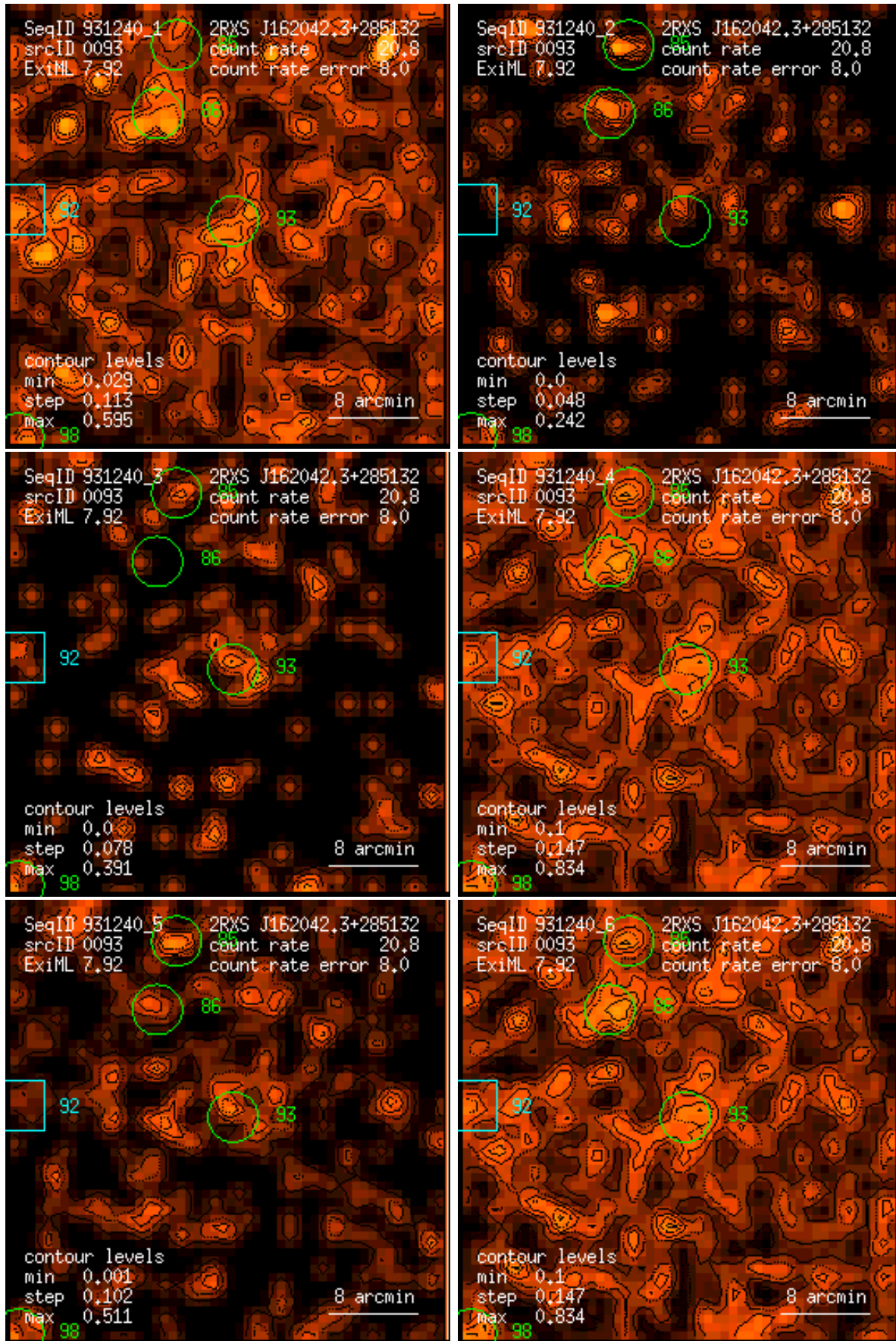
Figure 93: RASS 931240: detection 0093: band rate images, Gaussian filter: (1) PSPC channels 11 – 41, (2) 52 – 90, (3) 91 – 201, (4) 11 – 235, (5) 52 – 201, (6) 11 – 201. Broad band rates in counts/ks. Band rate contour levels in counts/ks/arcmin 2 .
