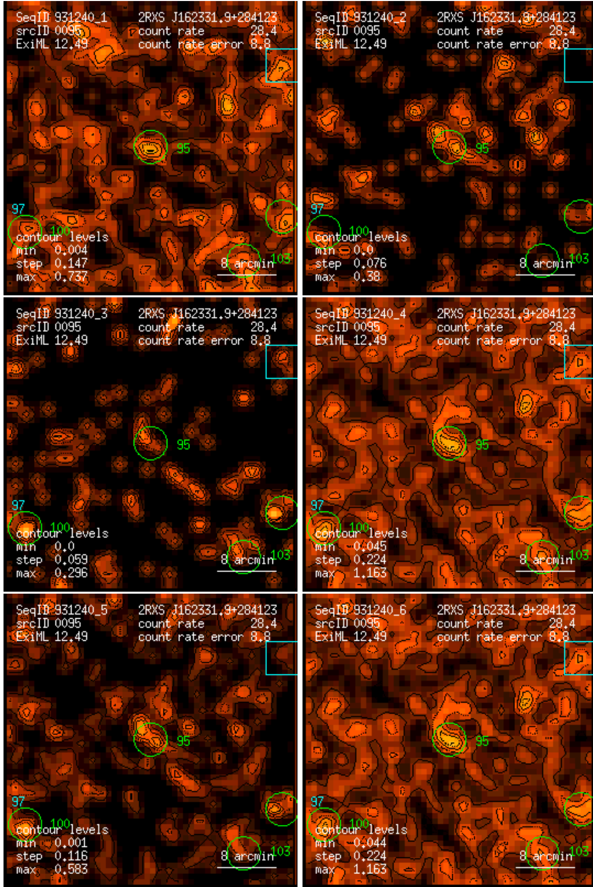
Figure 95: RASS 931240: detection 0095: band rate images, Gaussian filter: (1) PSPC channels 11 – 41, (2) 52 – 90, (3) 91 – 201, (4) 11 – 235, (5) 52 – 201, (6) 11 – 201. Broad band rates in counts/ks. Band rate contour levels in counts/ks/arcmin 2 .
