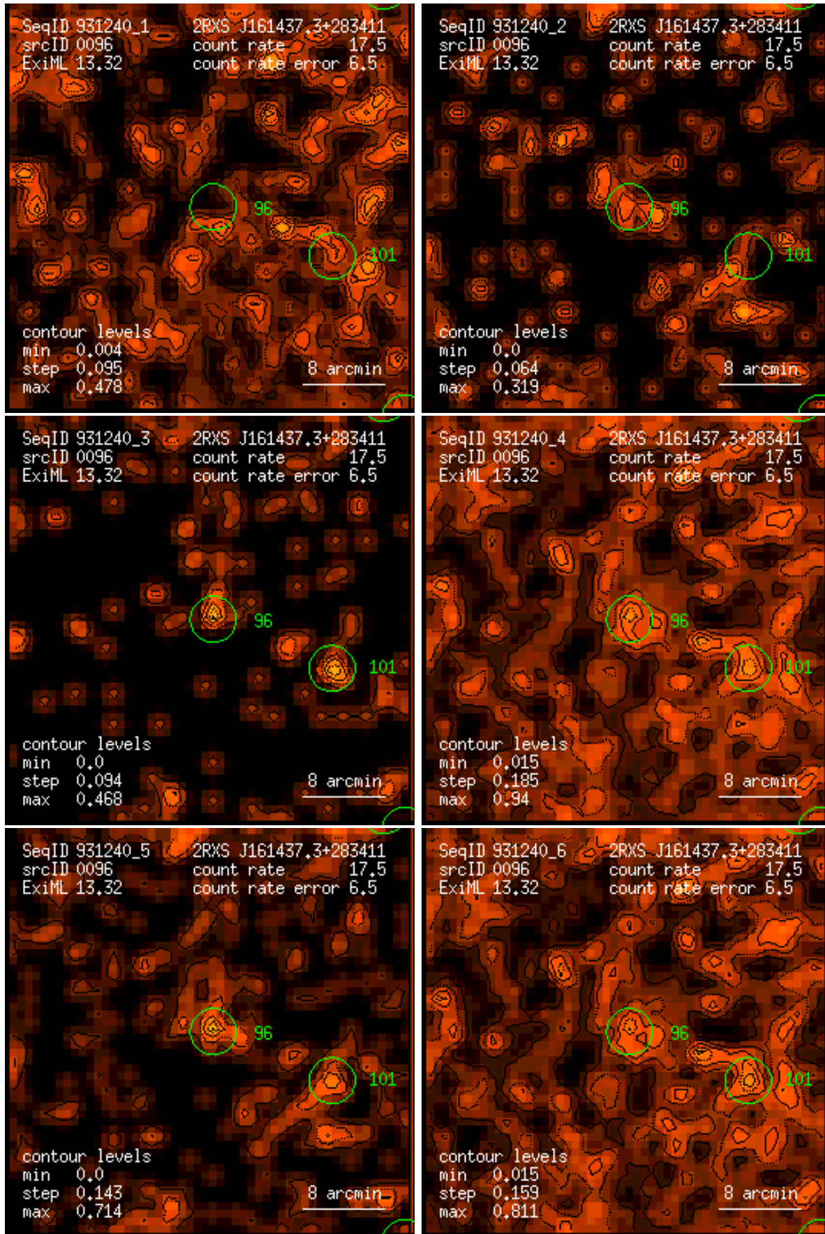
Figure 96: RASS 931240: detection 0096: band rate images, Gaussian filter: (1) PSPC channels 11 – 41, (2) 52 – 90, (3) 91 – 201, (4) 11 – 235, (5) 52 – 201, (6) 11 – 201. Broad band rates in counts/ks. Band rate contour levels in counts/ks/arcmin 2 .
