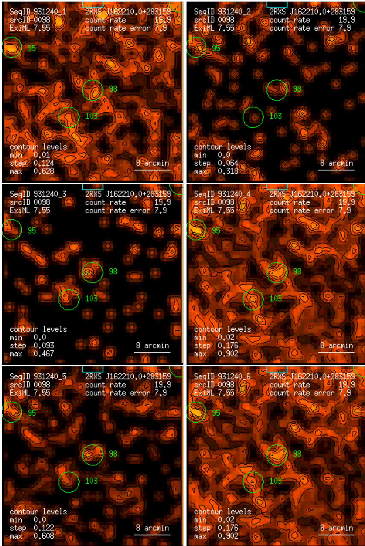
Figure 98: RASS 931240: detection 0098: band rate images, Gaussian filter: (1) PSPC channels 11 – 41, (2) 52 – 90, (3) 91 – 201, (4) 11 – 235, (5) 52 – 201, (6) 11 – 201. Broad band rates in counts/ks. Band rate contour levels in counts/ks/arcmin 2 .
