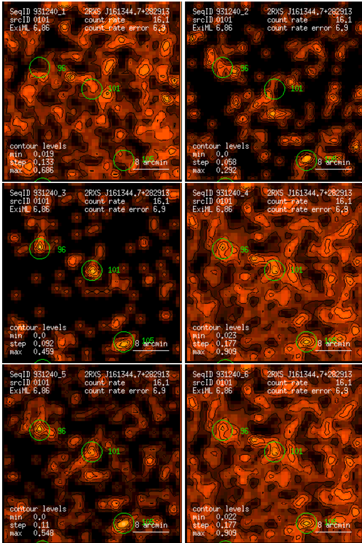
Figure 101: RASS 931240: detection 0101: band rate images, Gaussian filter: (1) PSPC channels 11 – 41, (2) 52 – 90, (3) 91 – 201, (4) 11 – 235, (5) 52 – 201, (6) 11 – 201. Broad band rates in counts/ks. Band rate contour levels in counts/ks/arcmin 2 .
