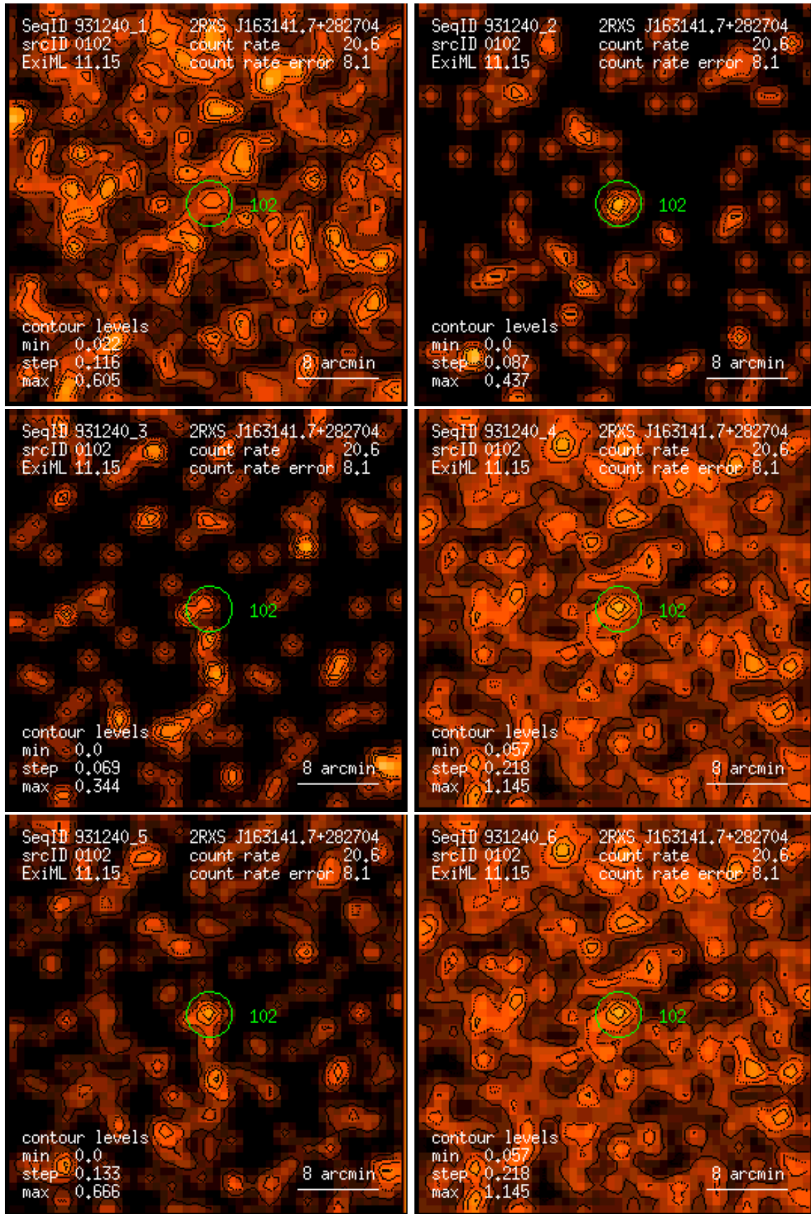
Figure 102: RASS 931240: detection 0102: band rate images, Gaussian filter: (1) PSPC channels 11 – 41, (2) 52 – 90, (3) 91 – 201, (4) 11 – 235, (5) 52 – 201, (6) 11 – 201. Broad band rates in counts/ks. Band rate contour levels in counts/ks/arcmin 2 .
