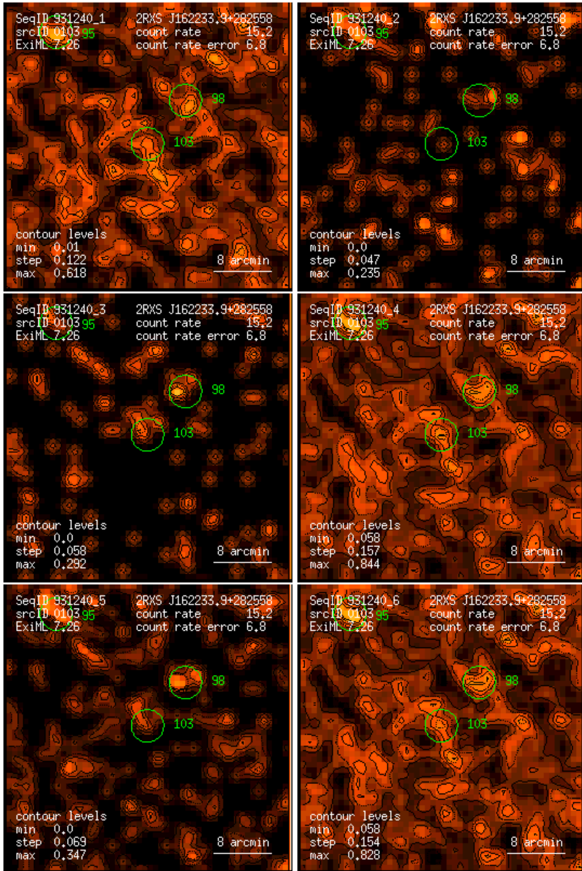
Figure 103: RASS 931240: detection 0103: band rate images, Gaussian filter: (1) PSPC channels 11 – 41, (2) 52 – 90, (3) 91 – 201, (4) 11 – 235, (5) 52 – 201, (6) 11 – 201. Broad band rates in counts/ks. Band rate contour levels in counts/ks/arcmin 2 .
