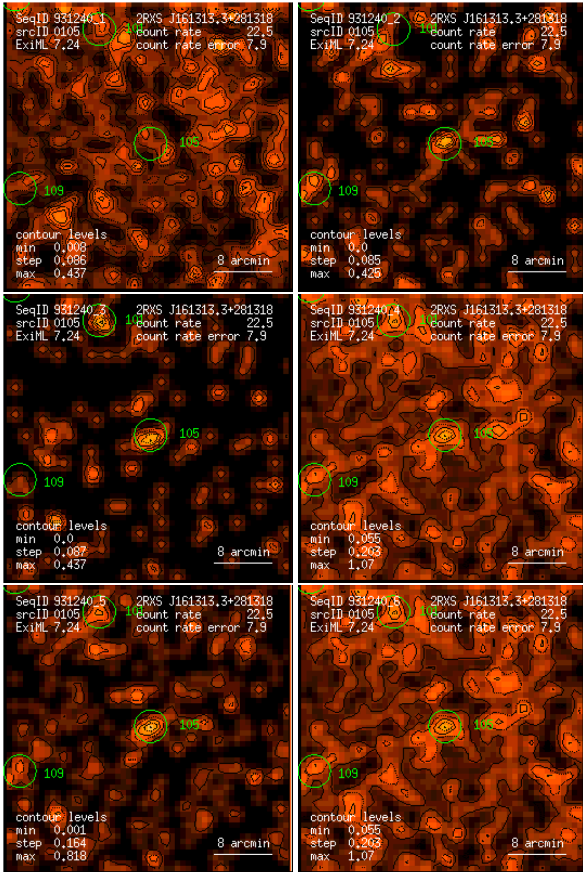
Figure 105: RASS 931240: detection 0105: band rate images, Gaussian filter: (1) PSPC channels 11 – 41, (2) 52 – 90, (3) 91 – 201, (4) 11 – 235, (5) 52 – 201, (6) 11 – 201. Broad band rates in counts/ks. Band rate contour levels in counts/ks/arcmin 2 .
