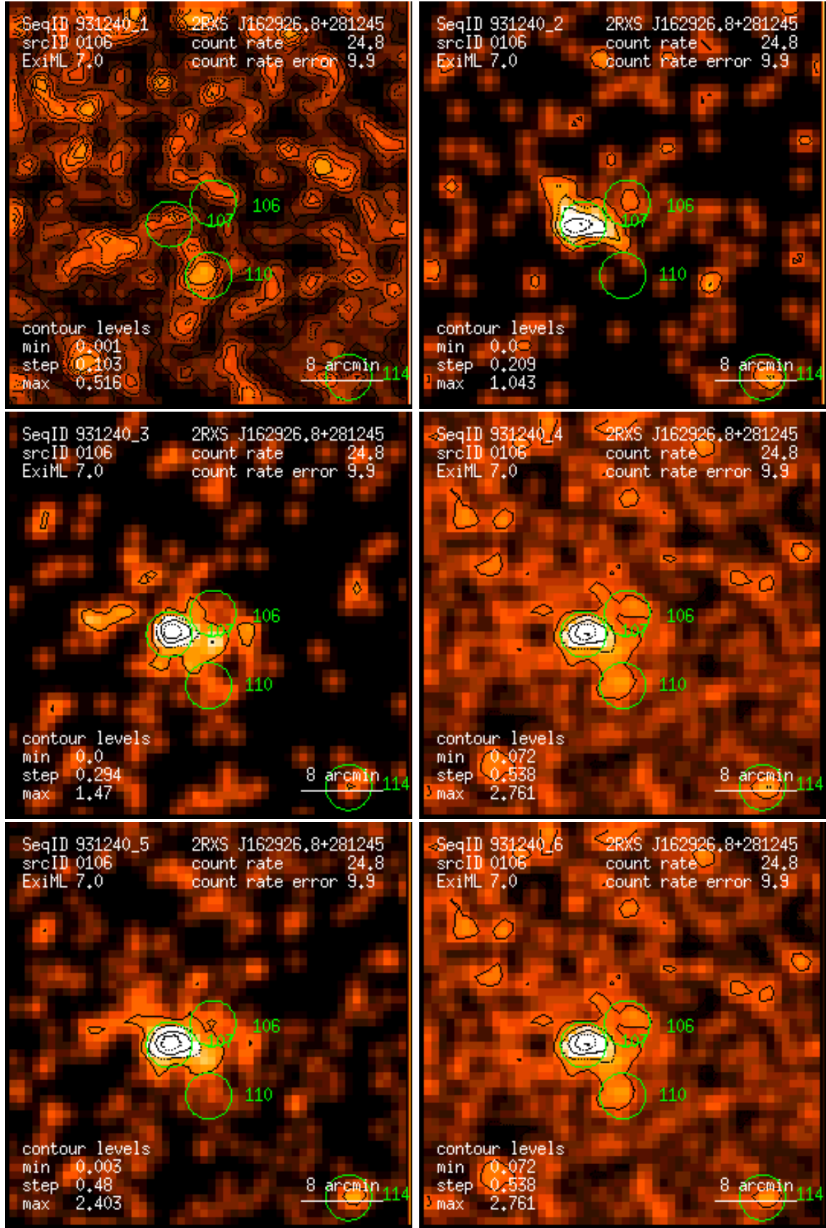
Figure 106: RASS 931240: detection 0106: band rate images, Gaussian filter: (1) PSPC channels 11 – 41, (2) 52 – 90, (3) 91 – 201, (4) 11 – 235, (5) 52 – 201, (6) 11 – 201. Broad band rates in counts/ks. Band rate contour levels in counts/ks/arcmin 2 .
