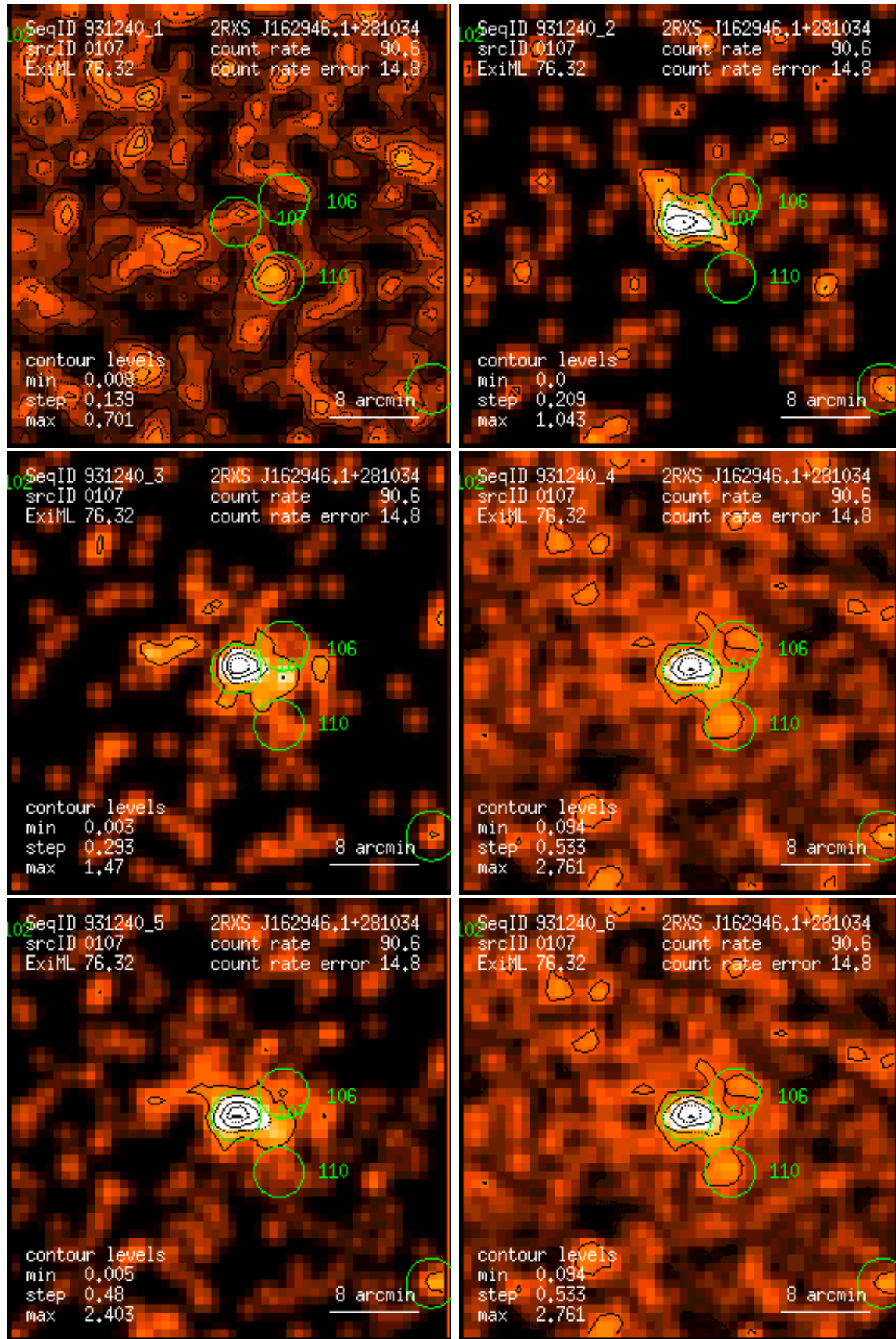
Figure 107: RASS 931240: detection 0107: band rate images, Gaussian filter: (1) PSPC channels 11 – 41, (2) 52 – 90, (3) 91 – 201, (4) 11 – 235, (5) 52 – 201, (6) 11 – 201. Broad band rates in counts/ks. Band rate contour levels in counts/ks/arcmin 2 .
