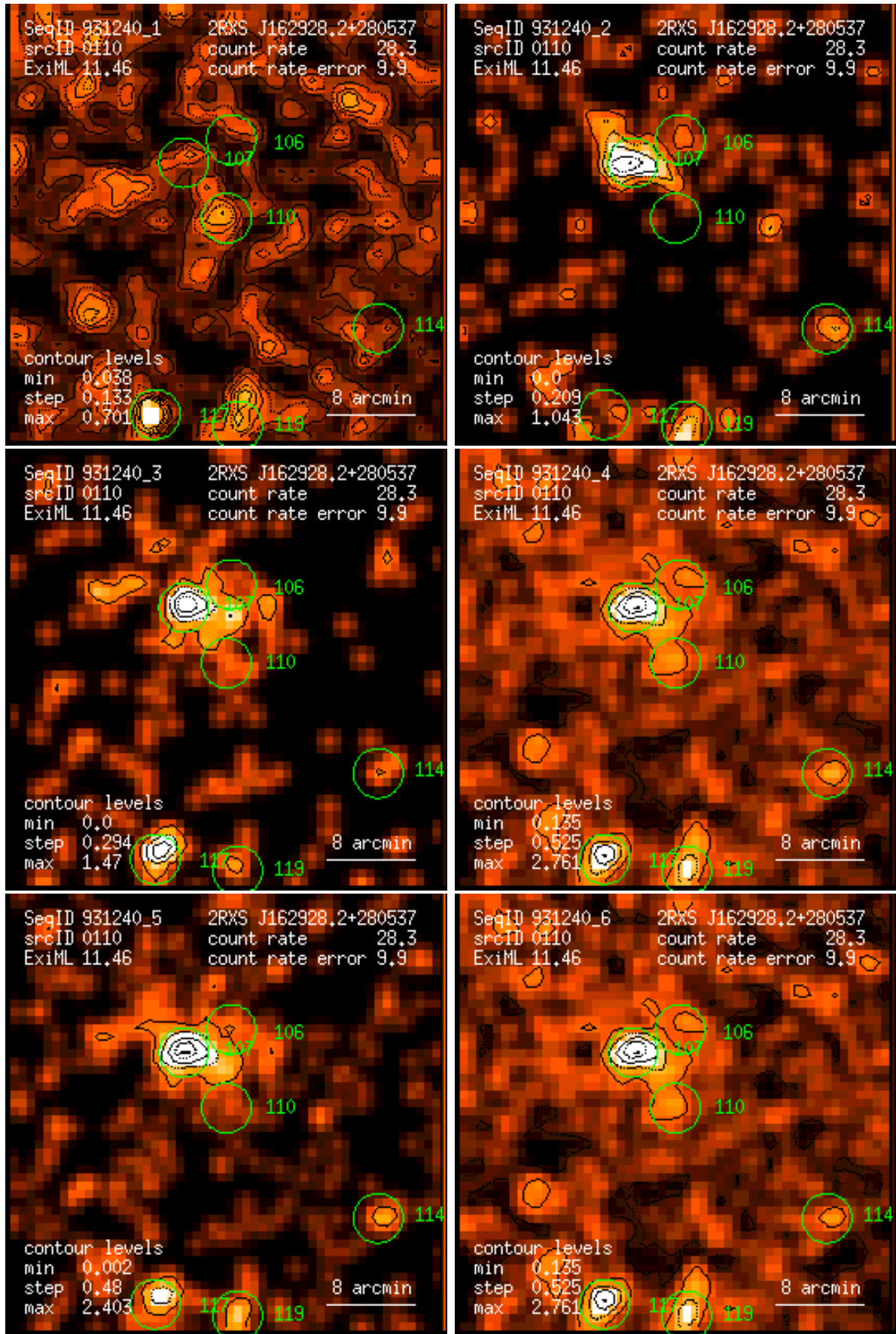
Figure 110: RASS 931240: detection 0110: band rate images, Gaussian filter: (1) PSPC channels 11 – 41, (2) 52 – 90, (3) 91 – 201, (4) 11 – 235, (5) 52 – 201, (6) 11 – 201. Broad band rates in counts/ks. Band rate contour levels in counts/ks/arcmin 2 .
