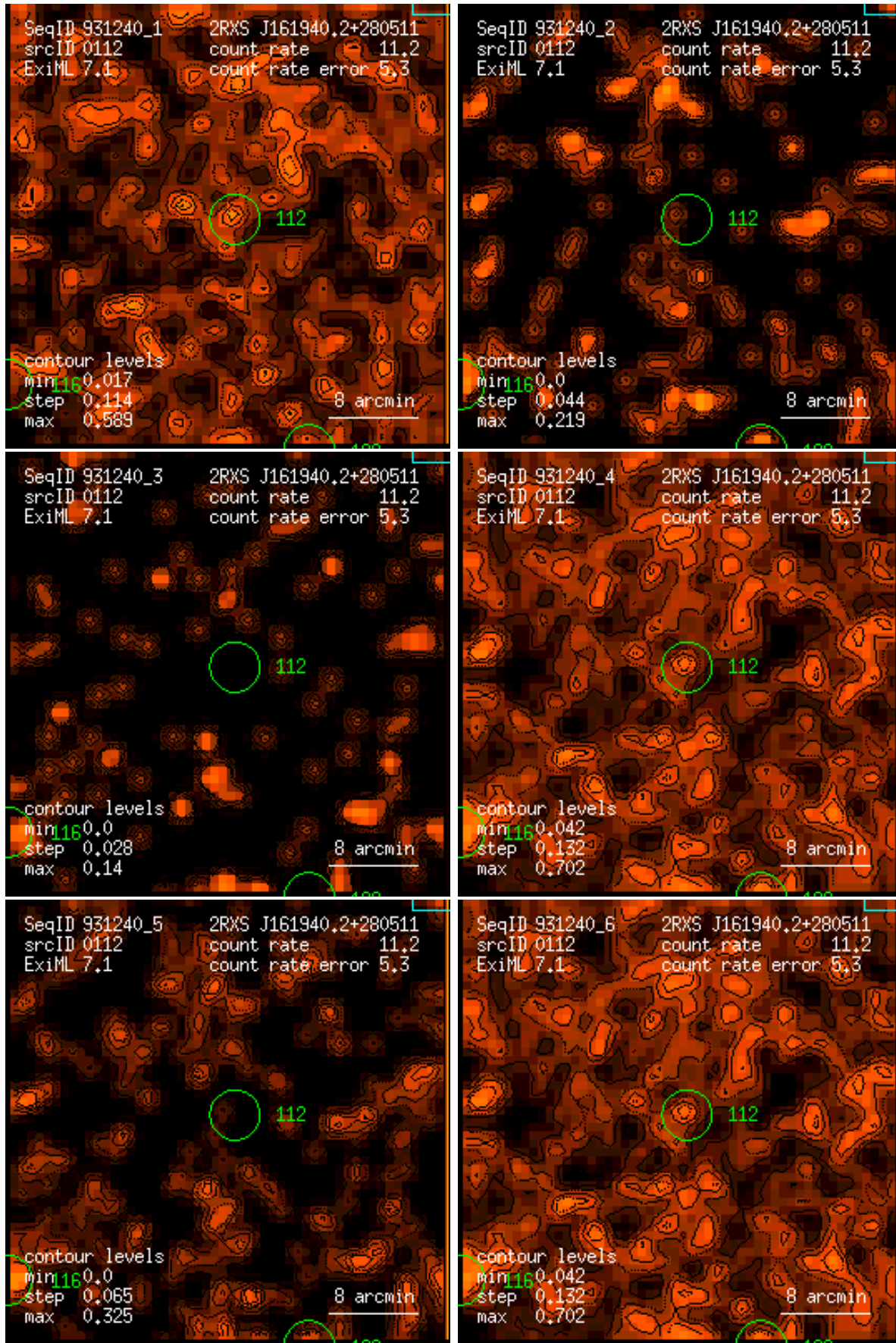
Figure 112: RASS 931240: detection 0112: band rate images, Gaussian filter: (1) PSPC channels 11 – 41, (2) 52 – 90, (3) 91 – 201, (4) 11 – 235, (5) 52 – 201, (6) 11 – 201. Broad band rates in counts/ks. Band rate contour levels in counts/ks/arcmin 2 .
