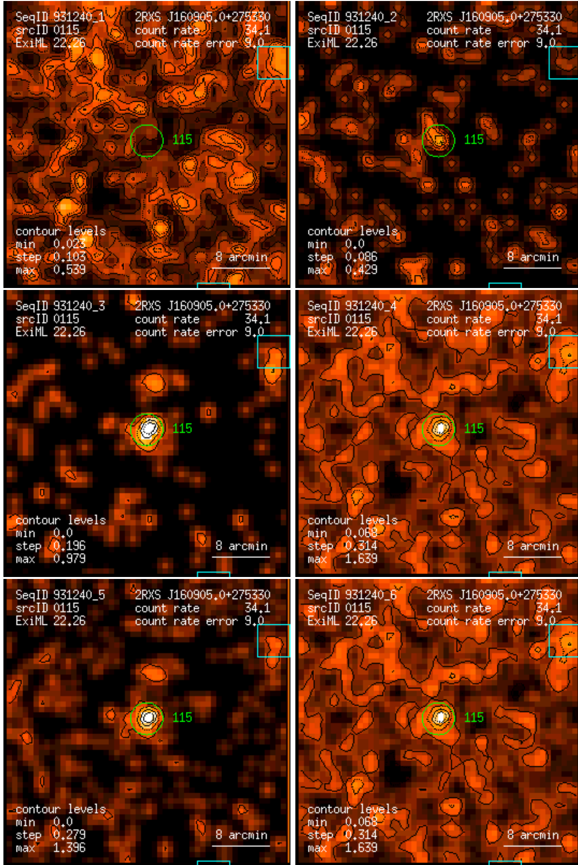
Figure 115: RASS 931240: detection 0115: band rate images, Gaussian filter: (1) PSPC channels 11 – 41, (2) 52 – 90, (3) 91 – 201, (4) 11 – 235, (5) 52 – 201, (6) 11 – 201. Broad band rates in counts/ks. Band rate contour levels in counts/ks/arcmin 2 .
