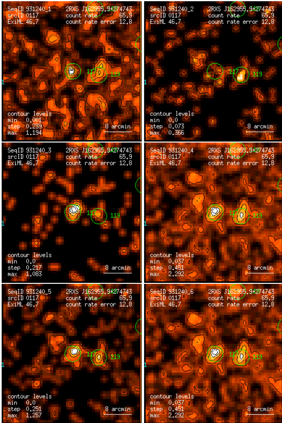
Figure 117: RASS 931240: detection 0117: band rate images, Gaussian filter: (1) PSPC channels 11 – 41, (2) 52 – 90, (3) 91 – 201, (4) 11 – 235, (5) 52 – 201, (6) 11 – 201. Broad band rates in counts/ks. Band rate contour levels in counts/ks/arcmin 2 .
