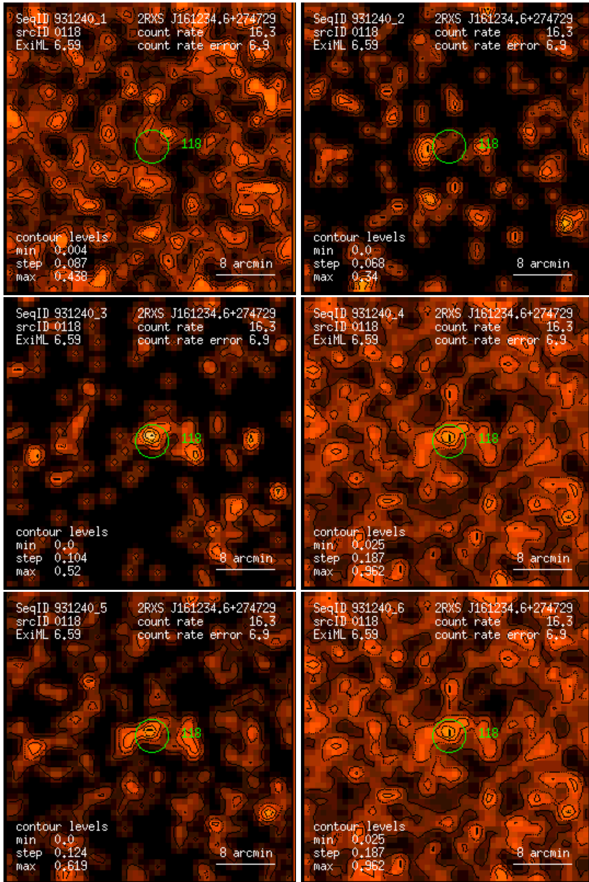
Figure 118: RASS 931240: detection 0118: band rate images, Gaussian filter: (1) PSPC channels 11 – 41, (2) 52 – 90, (3) 91 – 201, (4) 11 – 235, (5) 52 – 201, (6) 11 – 201. Broad band rates in counts/ks. Band rate contour levels in counts/ks/arcmin 2 .
