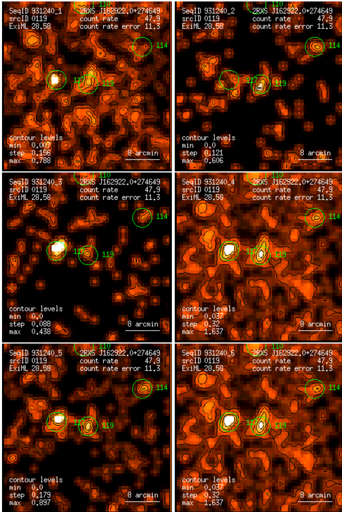
Figure 119: RASS 931240: detection 0119: band rate images, Gaussian filter: (1) PSPC channels 11 – 41, (2) 52 – 90, (3) 91 – 201, (4) 11 – 235, (5) 52 – 201, (6) 11 – 201. Broad band rates in counts/ks. Band rate contour levels in counts/ks/arcmin 2 .
