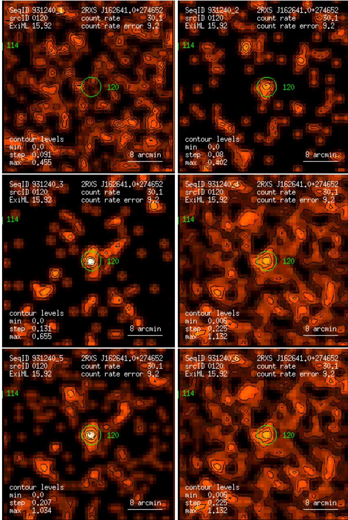
Figure 120: RASS 931240: detection 0120: band rate images, Gaussian filter: (1) PSPC channels 11 – 41, (2) 52 – 90, (3) 91 – 201, (4) 11 – 235, (5) 52 – 201, (6) 11 – 201. Broad band rates in counts/ks. Band rate contour levels in counts/ks/arcmin 2 .
