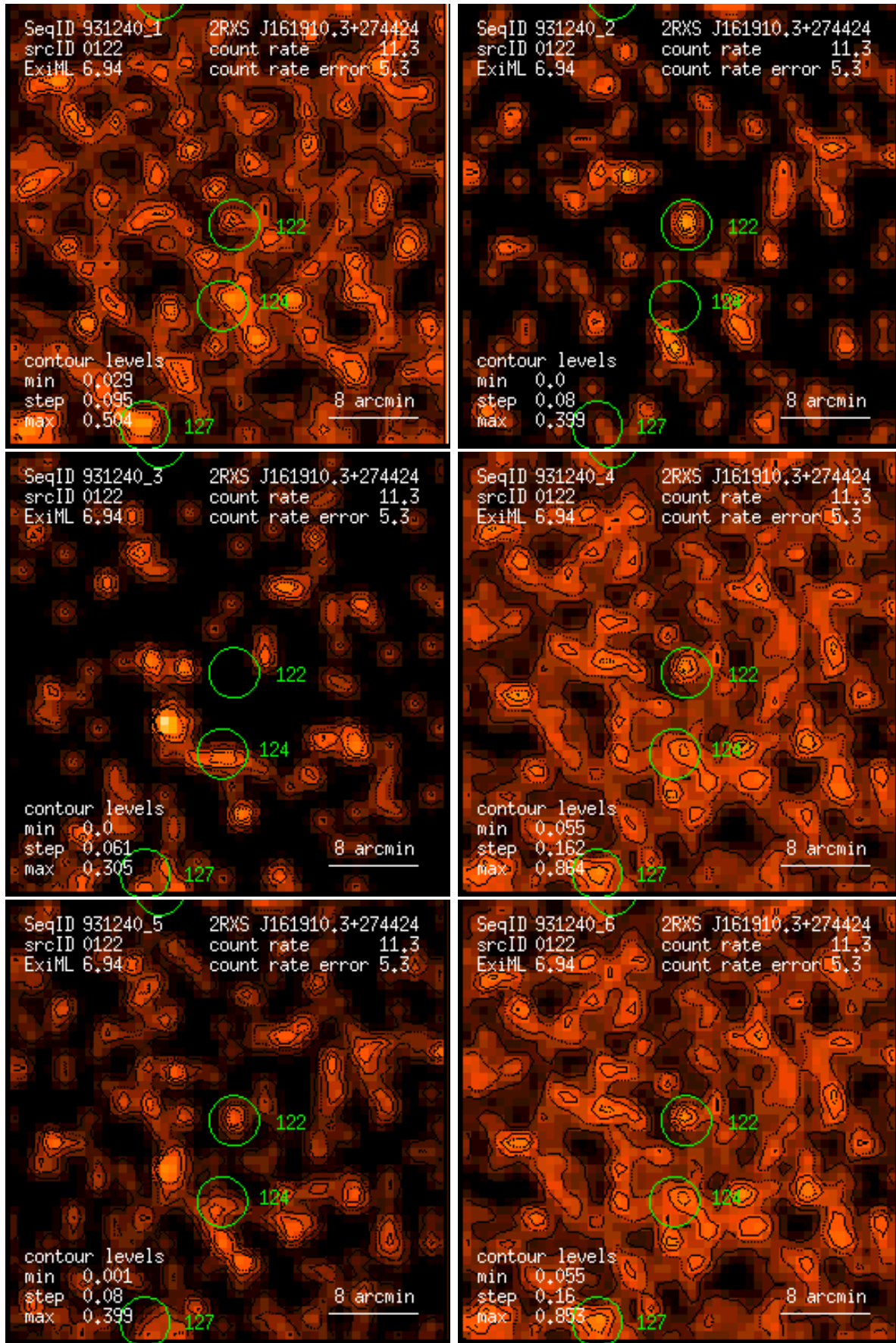
Figure 122: RASS 931240: detection 0122: band rate images, Gaussian filter: (1) PSPC channels 11 – 41, (2) 52 – 90, (3) 91 – 201, (4) 11 – 235, (5) 52 – 201, (6) 11 – 201. Broad band rates in counts/ks. Band rate contour levels in counts/ks/arcmin 2 .
