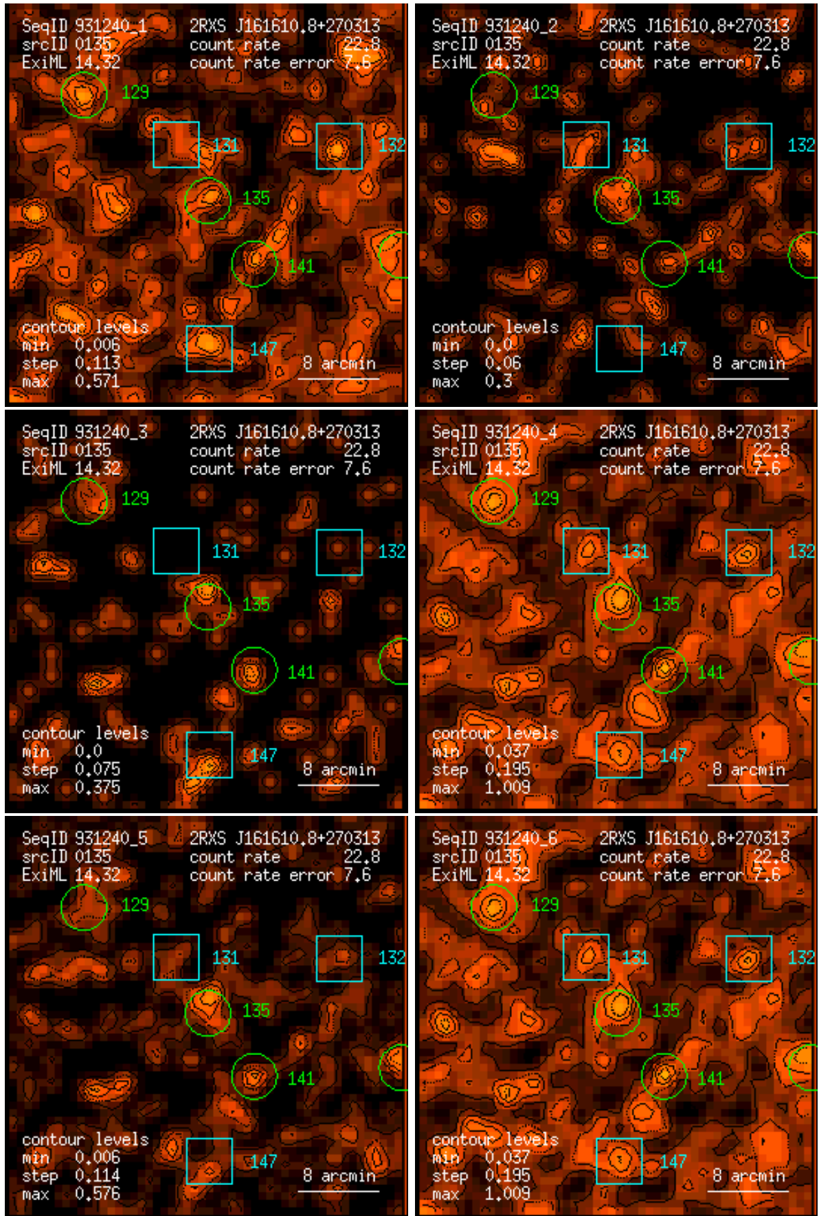
Figure 135: RASS 931240: detection 0135: band rate images, Gaussian filter: (1) PSPC channels 11 – 41, (2) 52 – 90, (3) 91 – 201, (4) 11 – 235, (5) 52 – 201, (6) 11 – 201. Broad band rates in counts/ks. Band rate contour levels in counts/ks/arcmin 2 .
