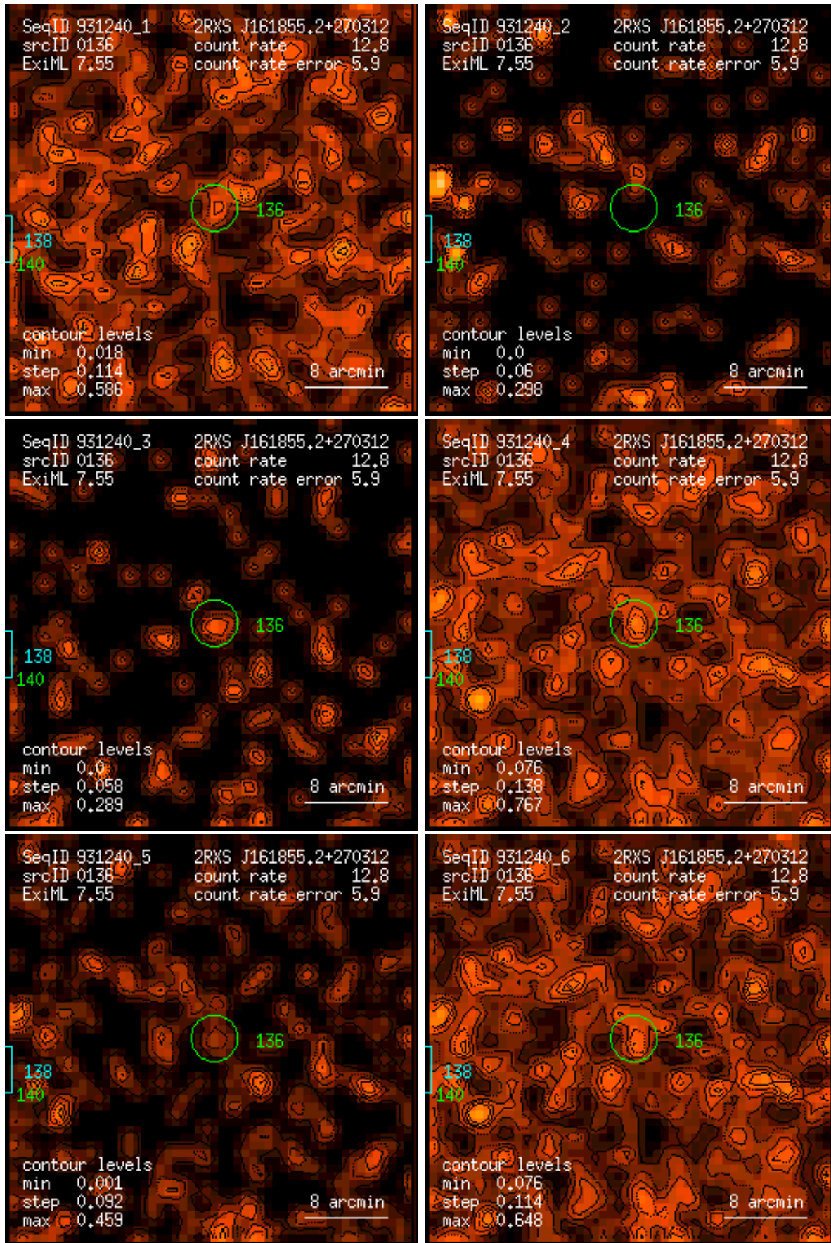
Figure 136: RASS 931240: detection 0136: band rate images, Gaussian filter: (1) PSPC channels 11 – 41, (2) 52 – 90, (3) 91 – 201, (4) 11 – 235, (5) 52 – 201, (6) 11 – 201. Broad band rates in counts/ks. Band rate contour levels in counts/ks/arcmin 2 .
