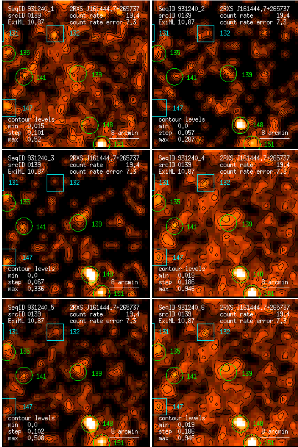
Figure 139: RASS 931240: detection 0139: band rate images, Gaussian filter: (1) PSPC channels 11 – 41, (2) 52 – 90, (3) 91 – 201, (4) 11 – 235, (5) 52 – 201, (6) 11 – 201. Broad band rates in counts/ks. Band rate contour levels in counts/ks/arcmin 2 .
