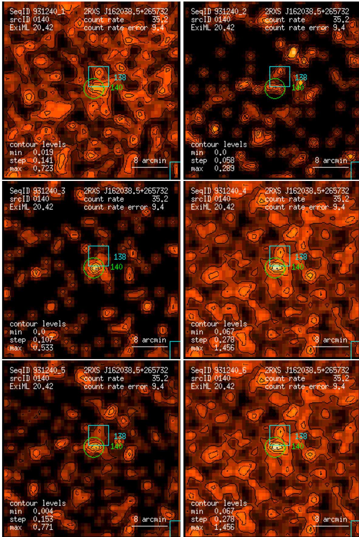
Figure 140: RASS 931240: detection 0140: band rate images, Gaussian filter: (1) PSPC channels 11 – 41, (2) 52 – 90, (3) 91 – 201, (4) 11 – 235, (5) 52 – 201, (6) 11 – 201. Broad band rates in counts/ks. Band rate contour levels in counts/ks/arcmin 2 .
