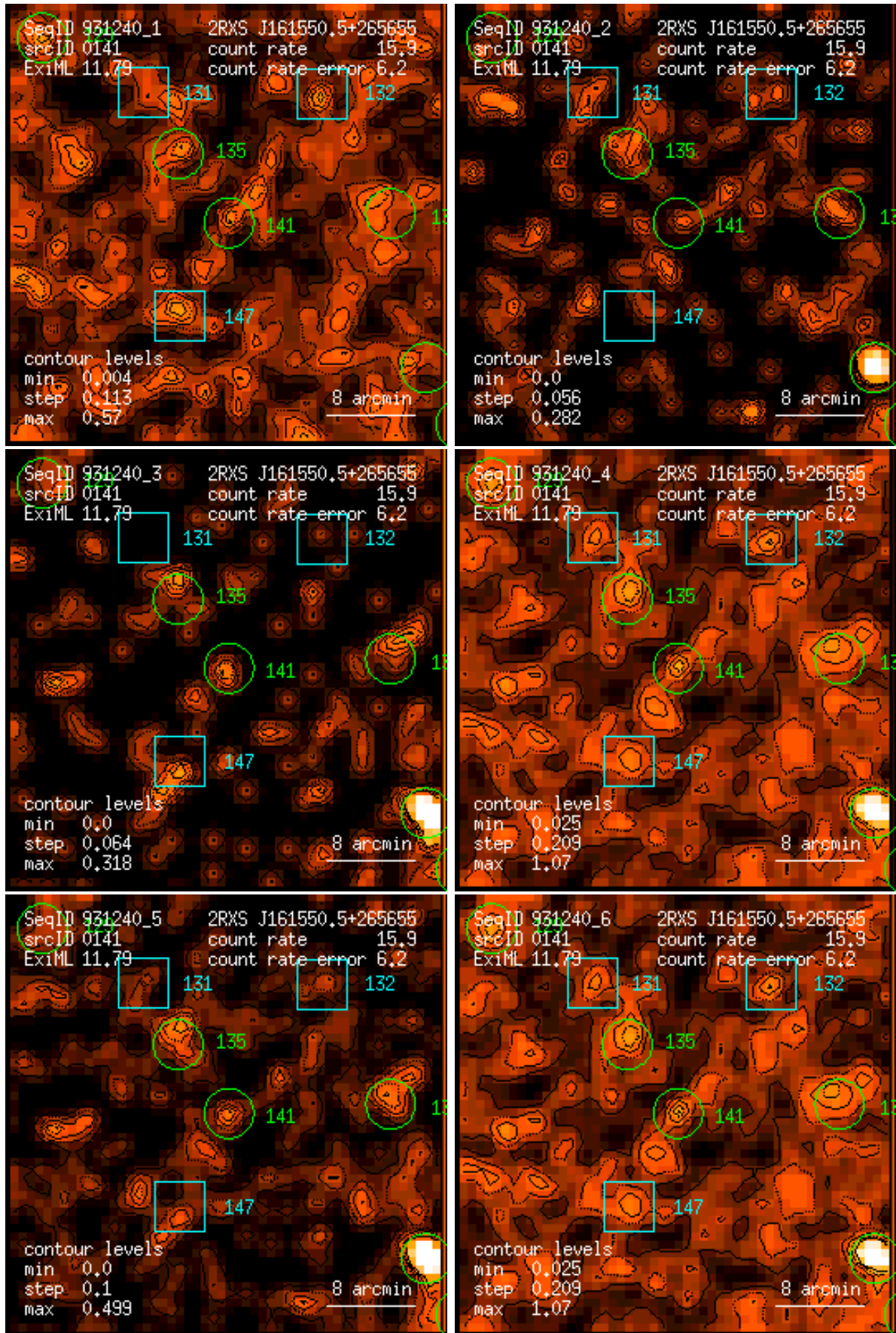
Figure 141: RASS 931240: detection 0141: band rate images, Gaussian filter: (1) PSPC channels 11 – 41, (2) 52 – 90, (3) 91 – 201, (4) 11 – 235, (5) 52 – 201, (6) 11 – 201. Broad band rates in counts/ks. Band rate contour levels in counts/ks/arcmin 2 .
