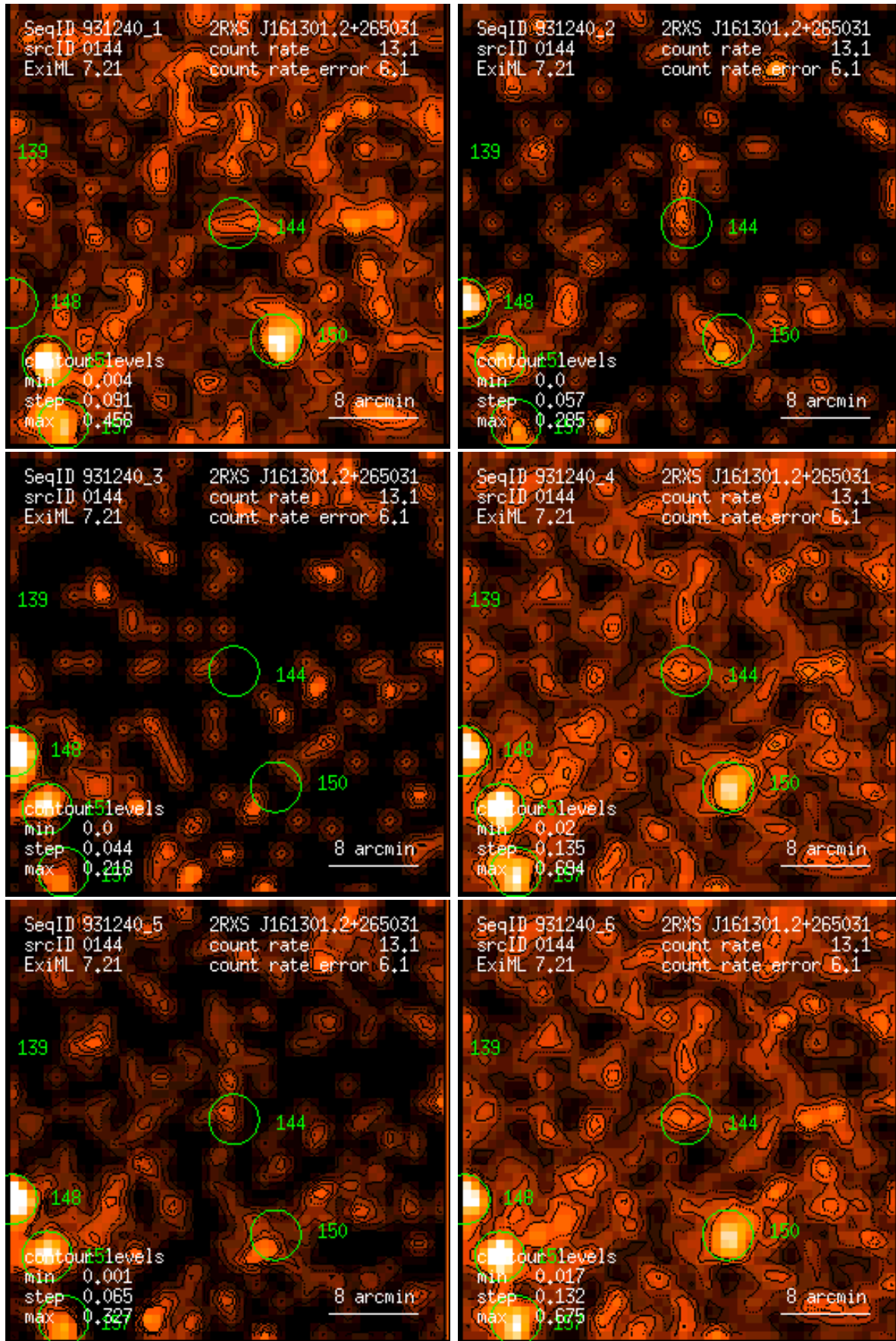
Figure 144: RASS 931240: detection 0144: band rate images, Gaussian filter: (1) PSPC channels 11 – 41, (2) 52 – 90, (3) 91 – 201, (4) 11 – 235, (5) 52 – 201, (6) 11 – 201. Broad band rates in counts/ks. Band rate contour levels in counts/ks/arcmin 2 .
