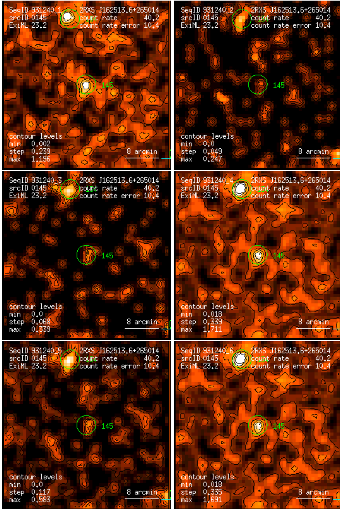
Figure 145: RASS 931240: detection 0145: band rate images, Gaussian filter: (1) PSPC channels 11 – 41, (2) 52 – 90, (3) 91 – 201, (4) 11 – 235, (5) 52 – 201, (6) 11 – 201. Broad band rates in counts/ks. Band rate contour levels in counts/ks/arcmin 2 .
