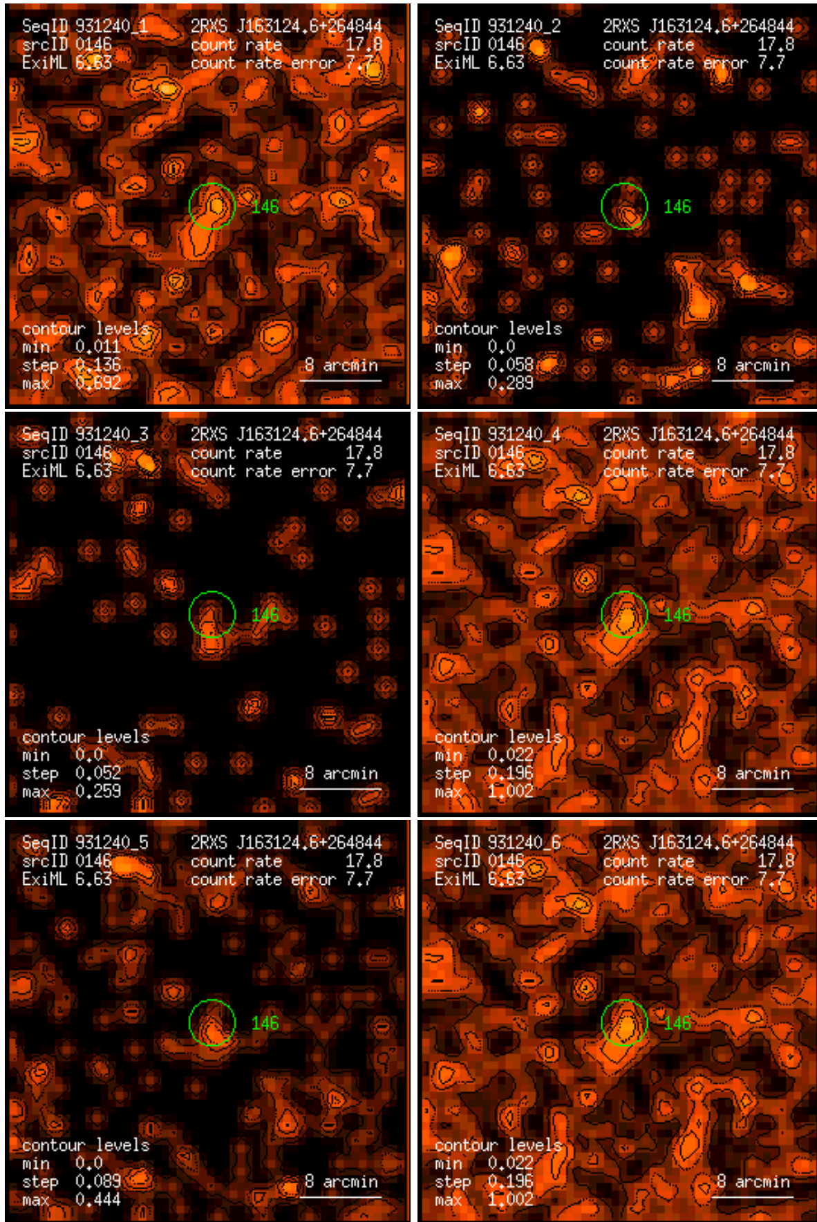
Figure 146: RASS 931240: detection 0146: band rate images, Gaussian filter: (1) PSPC channels 11 – 41, (2) 52 – 90, (3) 91 – 201, (4) 11 – 235, (5) 52 – 201, (6) 11 – 201. Broad band rates in counts/ks. Band rate contour levels in counts/ks/arcmin 2 .
