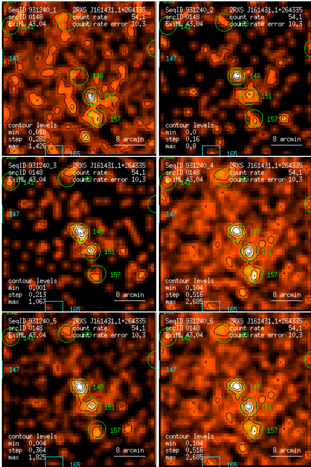
Figure 148: RASS 931240: detection 0148: band rate images, Gaussian filter: (1) PSPC channels 11 – 41, (2) 52 – 90, (3) 91 – 201, (4) 11 – 235, (5) 52 – 201, (6) 11 – 201. Broad band rates in counts/ks. Band rate contour levels in counts/ks/arcmin 2 .
