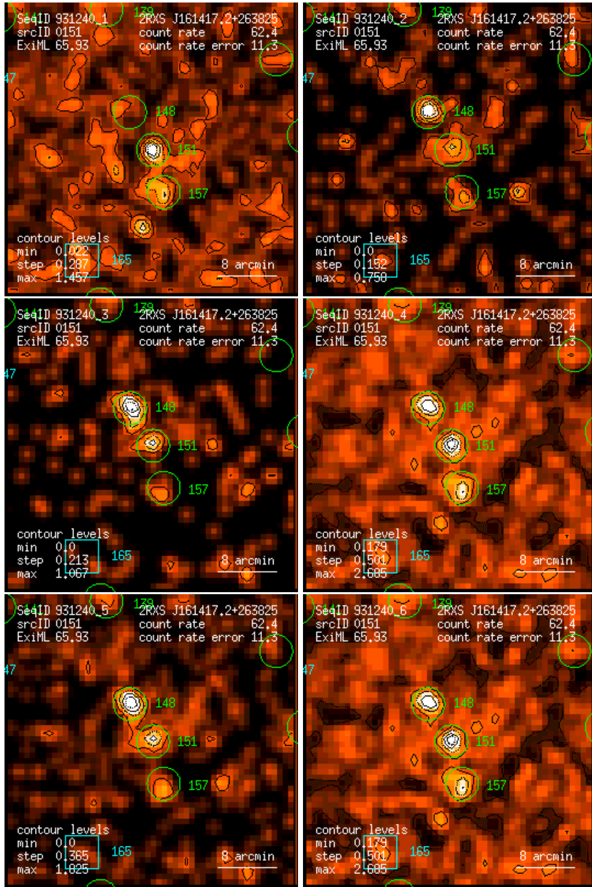
Figure 151: RASS 931240: detection 0151: band rate images, Gaussian filter: (1) PSPC channels 11 – 41, (2) 52 – 90, (3) 91 – 201, (4) 11 – 235, (5) 52 – 201, (6) 11 – 201. Broad band rates in counts/ks. Band rate contour levels in counts/ks/arcmin 2 .
