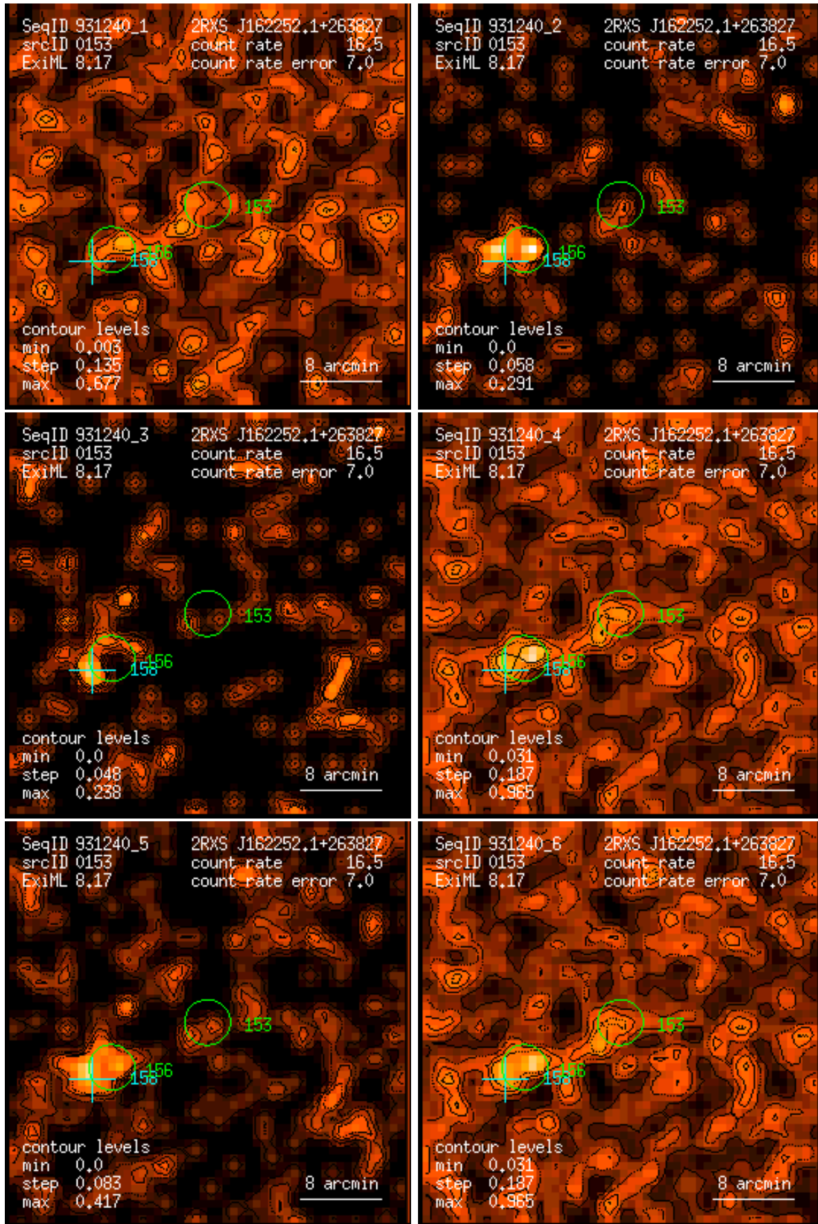
Figure 153: RASS 931240: detection 0153: band rate images, Gaussian filter: (1) PSPC channels 11 – 41, (2) 52 – 90, (3) 91 – 201, (4) 11 – 235, (5) 52 – 201, (6) 11 – 201. Broad band rates in counts/ks. Band rate contour levels in counts/ks/arcmin 2 .
