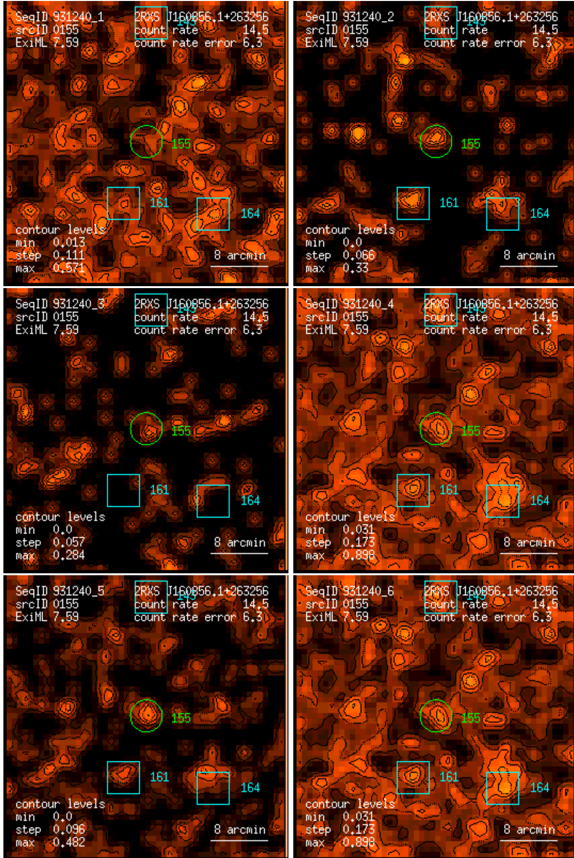
Figure 155: RASS 931240: detection 0155: band rate images, Gaussian filter: (1) PSPC channels 11 – 41, (2) 52 – 90, (3) 91 – 201, (4) 11 – 235, (5) 52 – 201, (6) 11 – 201. Broad band rates in counts/ks. Band rate contour levels in counts/ks/arcmin 2 .
