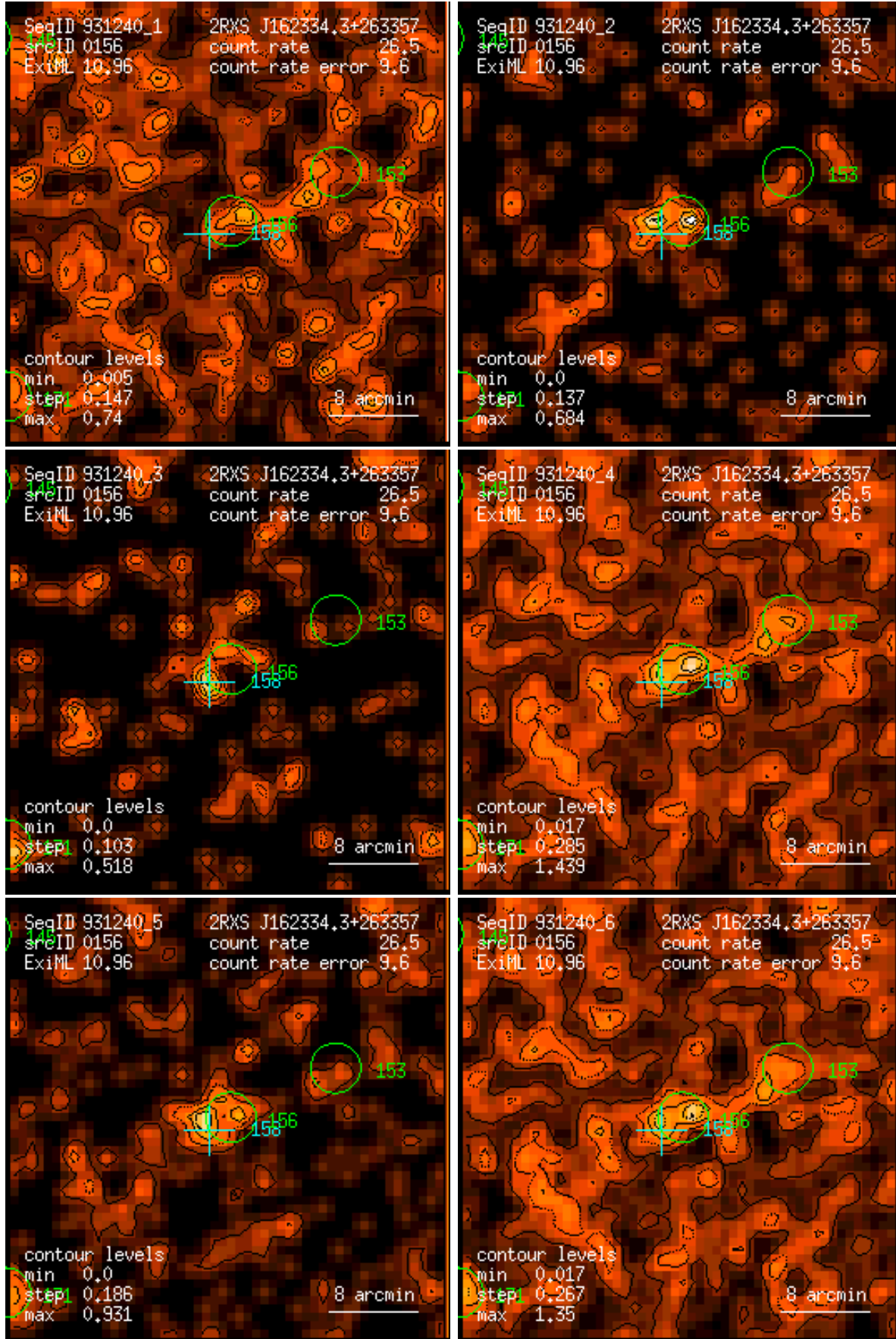
Figure 156: RASS 931240: detection 0156: band rate images, Gaussian filter: (1) PSPC channels 11 – 41, (2) 52 – 90, (3) 91 – 201, (4) 11 – 235, (5) 52 – 201, (6) 11 – 201. Broad band rates in counts/ks. Band rate contour levels in counts/ks/arcmin 2 .
