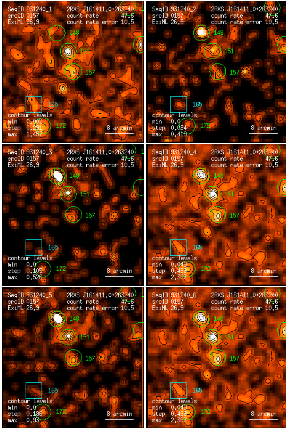
Figure 157: RASS 931240: detection 0157: band rate images, Gaussian filter: (1) PSPC channels 11 – 41, (2) 52 – 90, (3) 91 – 201, (4) 11 – 235, (5) 52 – 201, (6) 11 – 201. Broad band rates in counts/ks. Band rate contour levels in counts/ks/arcmin 2 .
