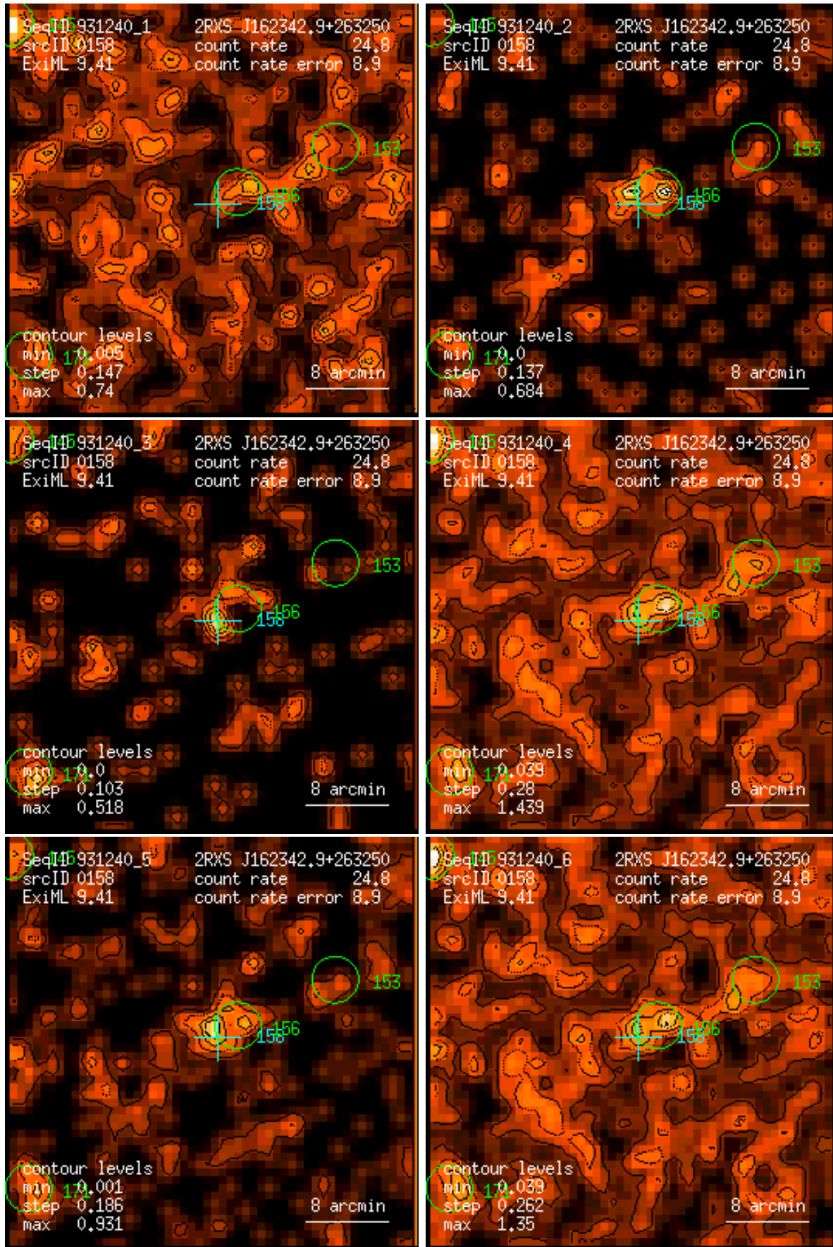
Figure 158: RASS 931240: detection 0158: band rate images, Gaussian filter: (1) PSPC channels 11 – 41, (2) 52 – 90, (3) 91 – 201, (4) 11 – 235, (5) 52 – 201, (6) 11 – 201. Broad band rates in counts/ks. Band rate contour levels in counts/ks/arcmin 2 .
