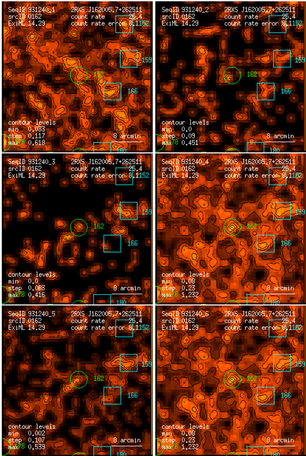
Figure 162: RASS 931240: detection 0162: band rate images, Gaussian filter: (1) PSPC channels 11 – 41, (2) 52 – 90, (3) 91 – 201, (4) 11 – 235, (5) 52 – 201, (6) 11 – 201. Broad band rates in counts/ks. Band rate contour levels in counts/ks/arcmin 2 .
